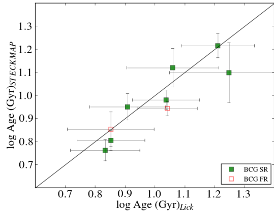
Figure 4. Comparison between STECKMAP and Lick estimated stellar populations. The green-filled squares represent the central stellar populations of the SR BCGs and the red-open squares represent the FR BCGs. The line shows the one-to-one relationship. The [\text{Fe}/\text{H}]_{[\alpha/\text{Fe}]=0} is equivalent to [\text{Z}/\text{H}] (see section 3.3). Our STECKMAP and Lick measurements agree within 1\sigma error.
