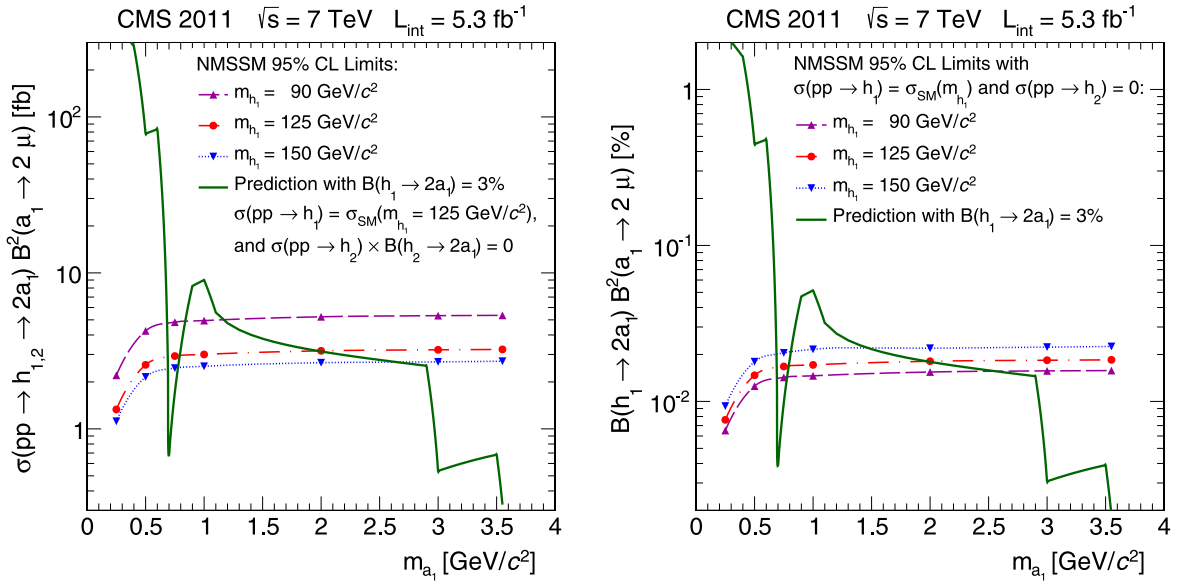
Fig. 3. Left: The 95% CL upper limits as functions of m_{a_1} , for the NMSSM case, on \sigma(pp \rightarrow h_{1,2} \rightarrow 2a_1) \times \mathcal{B}^2(a_1 \rightarrow 2\mu) with m_{h_1} = 90 GeV/ c^2 (dashed curve), m_{h_1} = 125 GeV/ c^2 (dash-dotted curve) and m_{h_1} = 150 GeV/ c^2 (dotted curve). The limits are compared to the predicted rate (solid curve) obtained using a simplified scenario with \mathcal{B}(h_1 \rightarrow 2a_1) = 3\% , \sigma(pp \rightarrow h_1) = \sigma_{SM}(m_{h_1} = 125 GeV/ c^2) [65], \sigma(pp \rightarrow h_2) \times \mathcal{B}(h_2 \rightarrow 2a_1) = 0 , and \mathcal{B}(a_1 \rightarrow 2\mu) as a function of m_{a_1} which is taken from [28] for NMSSM parameter \tan\beta = 20 . Right: The 95% CL upper limits on \mathcal{B}(h_1 \rightarrow 2a_1) \times \mathcal{B}^2(a_1 \rightarrow 2\mu) with m_{h_1} = 90 GeV/ c^2 (dashed curve), m_{h_1} = 125 GeV/ c^2 (dash-dotted curve) and m_{h_1} = 150 GeV/ c^2 (dotted curve) assuming \sigma(pp \rightarrow h_1) = \sigma_{SM}(m_{h_1}) [65] and \sigma(pp \rightarrow h_2) \times \mathcal{B}(h_2 \rightarrow 2a_1) = 0 . The limits are compared to the predicted branching fraction (solid line) obtained using a simplified scenario with \mathcal{B}(h_1 \rightarrow 2a_1) = 3\% and \mathcal{B}(a_1 \rightarrow 2\mu) as a function of m_{a_1} which is taken from [28] for NMSSM parameter \tan\beta = 20 .
