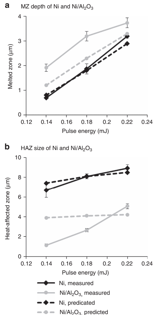
Figure 8 | Melted zone (MZ) depth and heat-affected zone (HAZ) size of Ni and Ni/Al 2 O 3 . Measured and predicted MZ depth ( a ) and HAZ size ( b ) of Ni and Ni/Al 2 O 3 at different pulse energies. As the pulse energy increases, the MZ and HAZ become larger for both materials. The MZ of Ni/Al 2 O 3 is larger than that of Ni, whereas the HAZ of Ni/Al 2 O 3 is much smaller than that of Ni at each energy level. The numerical model successfully predicts the effects (trends) introduced by nanoparticles on MZ and HAZ. The error bars in the measured MZ depths and HAZ sizes are the standard deviations calculated over five measurements.
