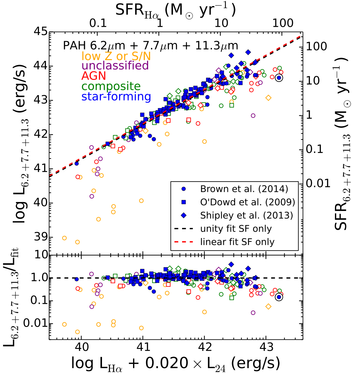
Figure 6. The top panel is the extinction-corrected H\alpha luminosity ( L_{H\alpha} + 0.020 \times L_{24 \mu\text{m}} ) versus total PAH luminosity ( L_{6.2 \mu\text{m}} + L_{7.7 \mu\text{m}} + L_{11.3 \mu\text{m}} PAH features). We fit a unity relation (dashed black line) to the primary calibration sample (filled blue points) and use this line (that we define as L_{\text{fit}} ) to show the ratio of the total PAH luminosity, for each galaxy, to the unity relationship as a function of extinction-corrected H\alpha luminosity (bottom panel). We classify galaxies as star-forming (filled blue points), composite (unfilled green points) or an AGN (unfilled red points) based on the location of their emission line ratios on a BPT diagram. Unclassified galaxies (unfilled purple points) did not have all lines required for BPT classification and the star-forming galaxies with low metallicity or S/N (unfilled orange points) are not used for the PAH SFR calibration (filled blue points; see text for more detail). The blue point enclosed by a black circle denotes II Zw 096, see § 4.4.
