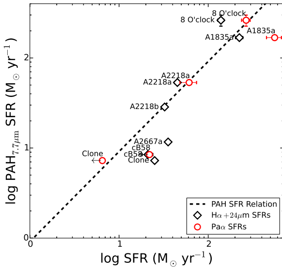
Figure 11. The estimated SFRs from the PAH 7.7 \mu m in comparison to the estimated Pa \alpha (open red circles) and H \alpha +24 \mu m (open black diamonds) SFRs for the demonstration sample (some of the statistical uncertainties are smaller than the symbol size, primarily for the vertical axis; see § 6.2 for discussion). The line shown is the unity PAH 7.7 \mu m SFR relation from our primary calibration sample (§ 4.1) to the Pa \alpha and H \alpha +24 \mu m SFR relations.
