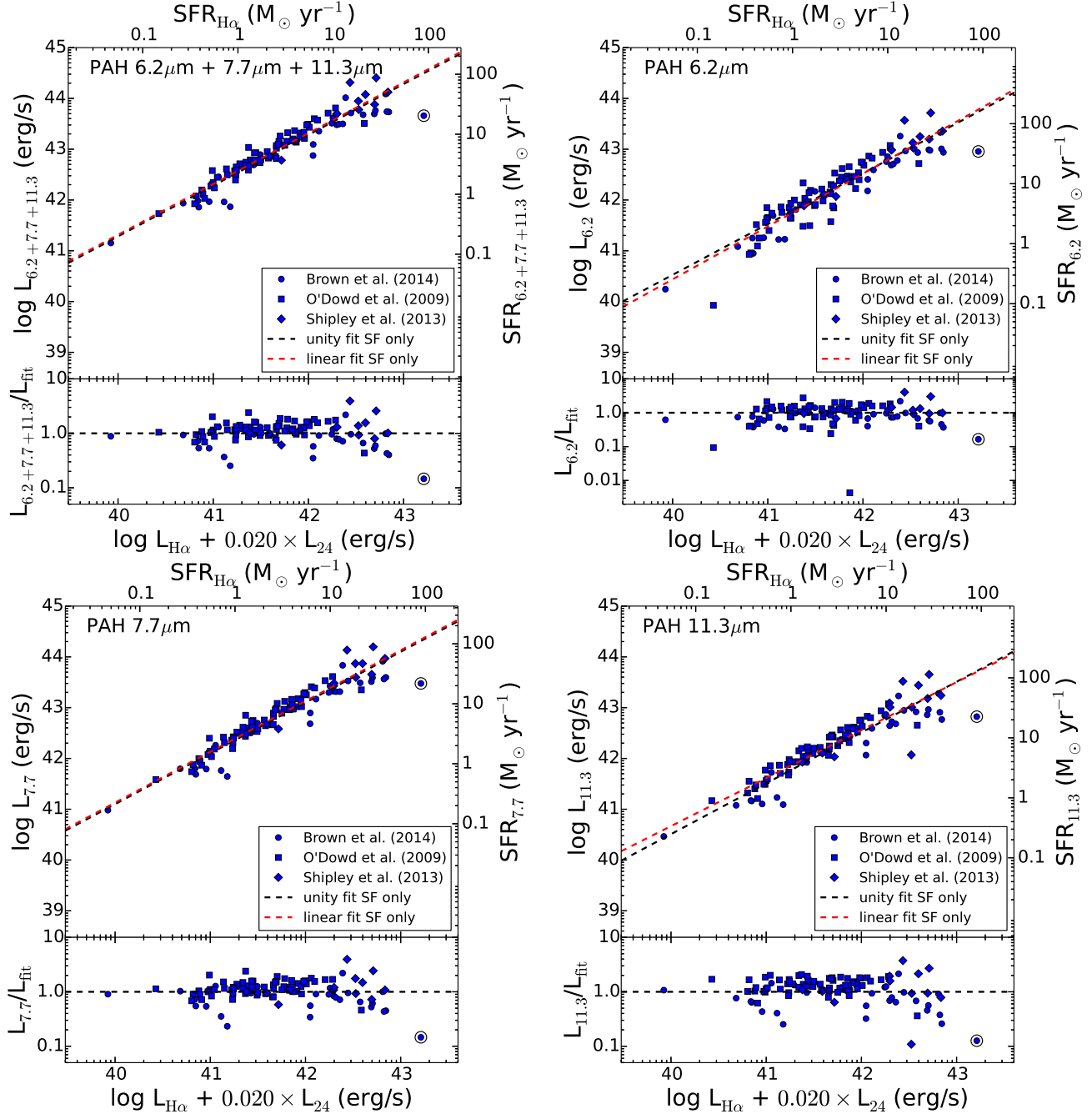
Figure 7. The extinction-corrected H\alpha luminosity ( L_{H\alpha} + 0.020 \times L_{24 \mu\text{m}} , Kennicutt et al. 2009) versus L_{\text{PAH}} (top left) and for the 6.2\mu\text{m} (top right), 7.7\mu\text{m} (bottom left) and 11.3\mu\text{m} (bottom right) PAH features separately. This illustrates that the small scatter persists for the individual PAH features ( \sigma_{\text{MAD}} \lesssim 0.2 dex). We fit a unity relation to the primary calibration sample (solid black line) and use this line as L_{\text{fit}} to determine residuals of expected L_{\text{PAH}} values (bottom for each panel). We used this fit to determine a SFR relation for L_{\text{PAH}} and each PAH feature shown individually (see § 4.1). The blue point enclosed by a black circle denotes II Zw 096, see § 4.4.
