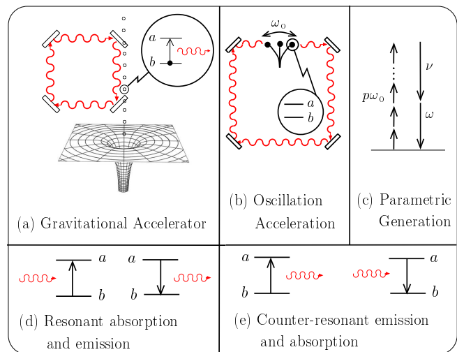
FIG. 1: (a) Atoms in the ground state |b\rangle are accelerated through small holes in the corner reflectors of a microwave (or optical) cavity by, e.g., a strong gravitational field. This is depicted as a unidirectional, single mode, ring cavity to convey the idea. (b) “Vibrating reed” piezoelectrically driven oscillator containing a two-level atom is placed in the cavity yielding strong maser action. (c) Parametric conversion of vibronic energy p\hbar\omega_0 into photon and atom energies \hbar\nu and \hbar\omega respectively. (d) An atom is excited (de-excited) as it simultaneously absorbs (emits) a photon in a resonant process. (e) The counter-resonant processes that are usually neglected as compared to the resonant processes in the “rotating wave” approximation; i.e. an atom is excited (de-excited) as it simultaneously emits (absorbs) a photon.
