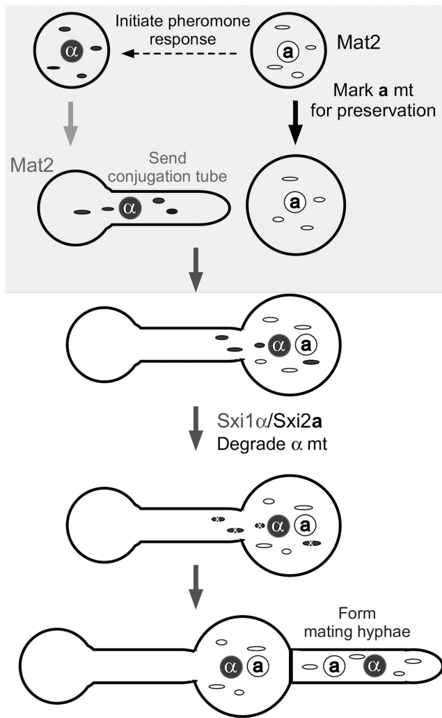
FIG 5 Model of mtDNA inheritance in Cryptococcus . Under mating-inducing conditions, the a cell activates Mat2 and produces high levels of the MFa pheromone (8). In response to MFa , the \alpha cell activates Mat2 and produces a conjugation tube. The earlier induction of Mat2 at a higher level in the a cell marks its mitochondria for preservation. Immediately after cell fusion, the Sxi1 \alpha /Sxi2a complex forms, and it helps degrade the unprotected \alpha mitochondria in the newly formed zygote. Thus, the a mitochondria dominate in the mature zygote and cells subsequently generated from that zygote (e.g., hyphae and spores).
