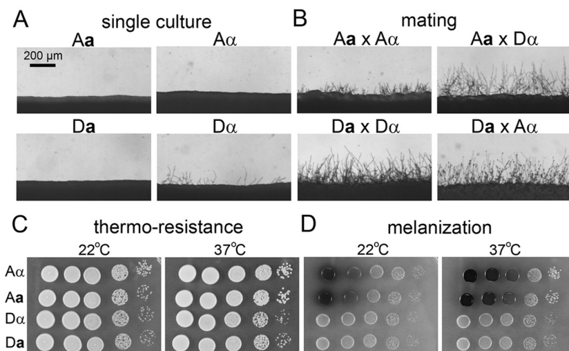
FIG 2 Phenotypic differences of the strains used. (A) Strains were incubated alone on V8 agar medium for 48 h. A and D represent variety serotype A and serotype D, respectively. a and \alpha indicate the mating types of the strains. (B) Coculture of cells of opposite mating types on a V8 agar plate for 48 h to visualize filamentation, which reflects successful mating. (C and D) Strains with equal numbers of cells with serial dilutions were inoculated on YPD medium (C) or L-DOPA medium (D) and incubated at the indicated temperature for 48 h to analyze their thermotolerance and melanin production, respectively.
