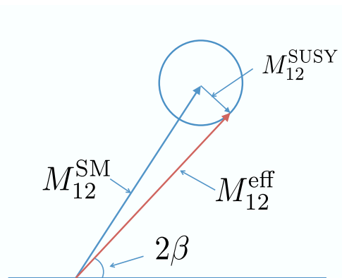
FIG. 2: The illustration of the SM and SUSY contribution of the mixing amplitude of B - \bar{B} mixing in the complex plane. The detail is explained in the text.
