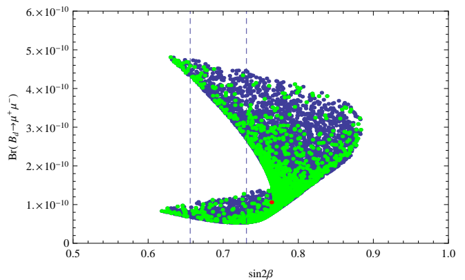
FIG. 3: We show the correlation between B_d \rightarrow \mu^+ \mu^- and B_d - \bar{B}_d mixing for the choice of SUSY parameters described in the text. The blue plots are for the randomly generated a, b, c in the anti-symmetric coupling, and the green points satisfy all the experimental data, such as K - \bar{K} mixing, B_s - \bar{B}_s mixing, and b \rightarrow d\gamma , b \rightarrow s\gamma . The red point shows the SM prediction. The dashed lines show the 2\sigma region of the experimental measurement of \sin 2\beta .
