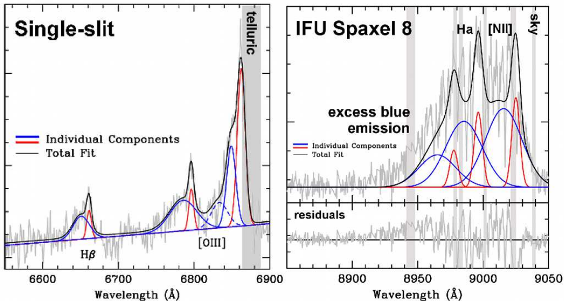
Figure 2. Left: Single-slit spectrum centered on the nucleus of S1 ( z = 0.3692 \pm 0.0002 ). The line-of-sight velocity offsets are \sim \pm 200 \text{ km s}^{-1} and FWHM line-widths are 200 - 1000 \text{ km s}^{-1} for the main red and blue components. The red side of the [\text{OIII}]\lambda 5007 line is affected by telluric absorption. Forcing consistency between the profile shapes for the \text{H}\beta and [\text{OIII}]\lambda 4959 lines requires an additional broad component blueshifted by 900 \text{ km s}^{-1} on the [\text{OIII}]\lambda 5007 line; this broad component is below our detection limit for \text{H}\beta and [\text{OIII}]\lambda 4959 . The total fit is offset slightly high. Right: Excess blue emission, seen after applying a two component model, indicates that the second blueshifted component (seen on the [\text{OIII}]\lambda 5007 line in 1) is necessary.
