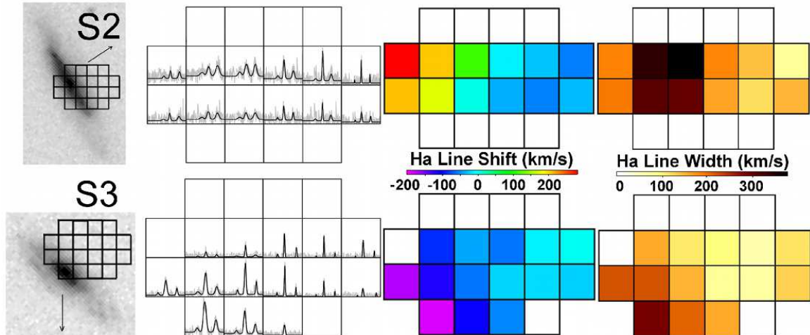
Figure 3. HST/ACS F814W image with the FLAMES/GIRAFFE IFU footprint ( 3'' \times 2'' = 15 \text{ kpc} \times 10 \text{ kpc} ) overlaid for sources SG1120-S2 and SG1120-S3. We center the IFU spaxel with the largest continuum value on the nucleus of the galaxy. The IFU footprint is populated with the spectra for each spaxel centered on the [NII] & H \alpha lines. The data are shown in light grey and our fit to the emission lines in black. Line shift and line width maps are shown. Errors on the line shifts (widths) are 68 \text{ km s}^{-1} ( 5 - 15 \text{ km s}^{-1} ) and 73 \text{ km s}^{-1} ( 5 \text{ km s}^{-1} ) for sources S2 and S3, respectively, following from the \sim 100 \text{ km s}^{-1} errors on the systemic velocity. Arrows indicate the direction toward the nearest group center, G4 for S2 and G2 for S3; group properties are detailed in Gonzalez et al. (2005) and Tran et al. (2009). Both S2 and S3 have extraplanar gas to at least r_h \sim 10 \text{ kpc} above their disks.
