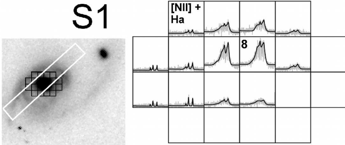
Figure 1. Left: HST/ACS F814W image with the FLAMES/GIRAFFE IFU ( 3'' \times 2'' = 15 \text{ kpc} \times 10 \text{ kpc} ) and single-slit ( 1'' ) footprints overlaid for source SG1120-S1. Right: The IFU data for S1 with spaxel 8 indicated.
