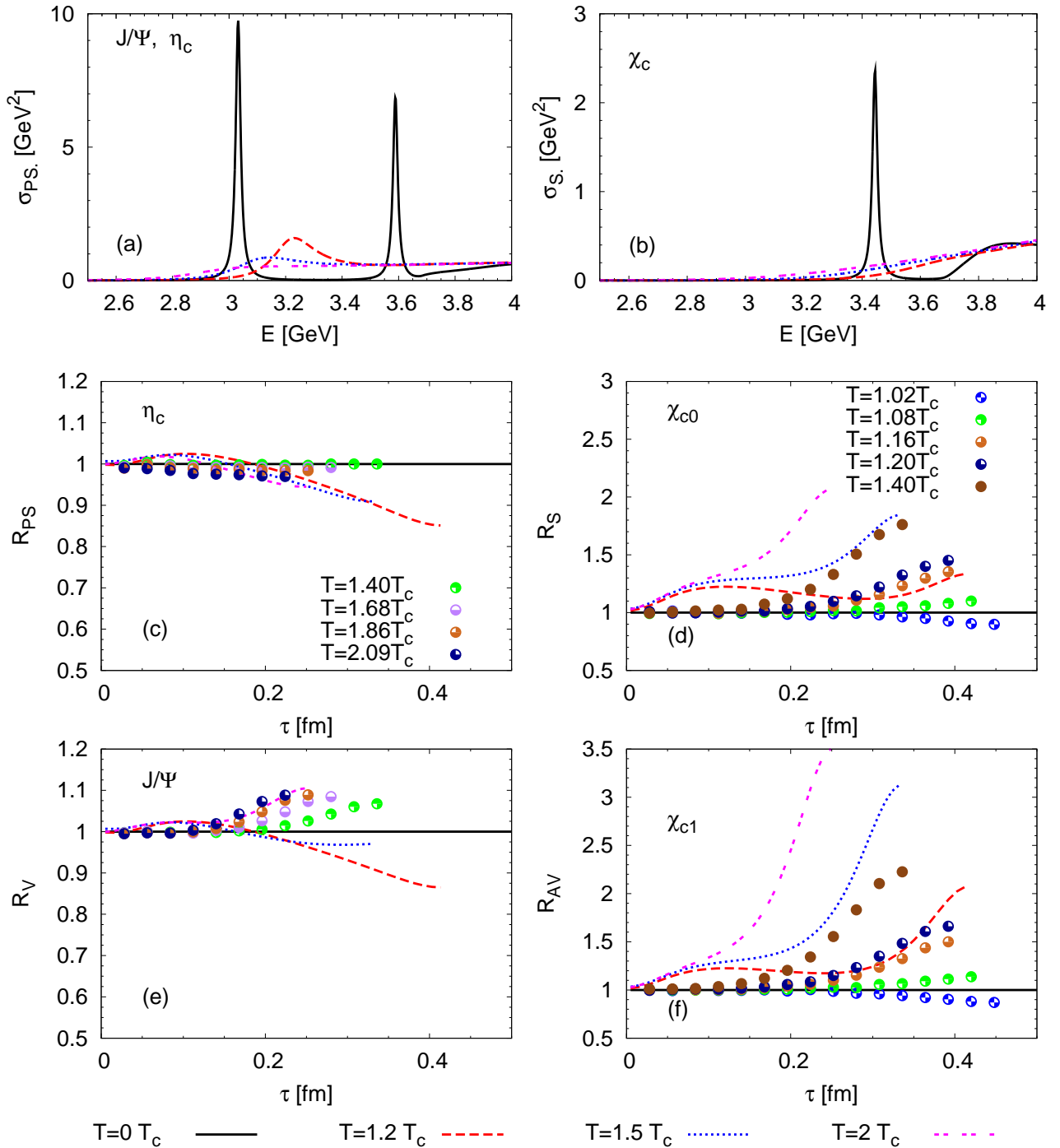
FIG. 1: (Color online) Charmonium spectral functions in the pseudoscalar (upper left panel) and scalar (upper right) channel for different temperatures using the internal energy, U , as Q\bar{Q} potential. In the middle and lower rows we show the corresponding euclidean correlator ratios in the pseudoscalar (middle left), scalar (middle right), vector (lower left) and axialvector channels (lower right), where the latter three include zero-mode contribution. The comparison to the lattice data (indicated by symbols) [35] is made in absolute units of \tau (limited to 1/2T at each temperature), with T_c \simeq 210 MeV for the lattice data and T_c \simeq 196 MeV underlying the potential for the T -matrix calculations (e.g., 1.4 T_c^{\text{lat}} \simeq 1.5 T_c^{\text{Tmat}} ).
