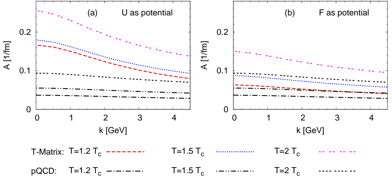
FIG. 4: (Color online) Charm-quark relaxation rate as a function of 3-momentum for different temperatures using either the T -Matrix plus pQCD gluon scattering [10] (upper 3 lines in left panel) or a pQCD calculation for scattering off gluons and anti/quarks (lower 3 lines in left panel). The T -matrix is computed using U (left) or F (right) as potential while pQCD contributions are obtained with \alpha_s=0.4 .
