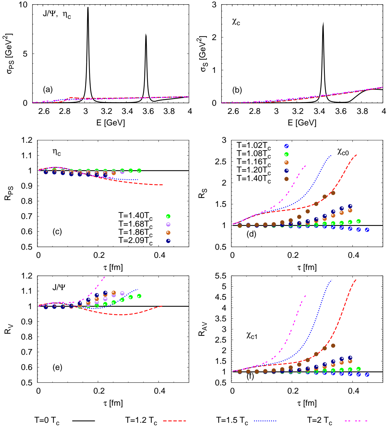
FIG. 2: (Color online) Same as Fig. 1 but using the free energy, F , as Q\bar{Q} potential.
