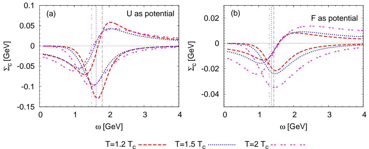
FIG. 3: (Color online) Real and imaginary parts of the charm-quark selfenergy at vanishing 3-momentum in a QGP at different temperatures for the scenarios where the internal (left panel) or free energy (right panel) is employed as potential. The imaginary parts are negative definite while the real parts change sign close to the vertical lines which indicate the effective charm-quark mass (on-shell energy) at the respective temperature.
