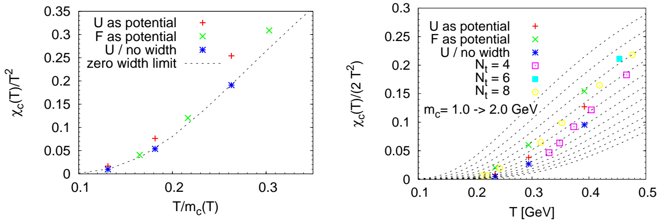
FIG. 5: (Color online) Charm-quark number susceptibility as a function of temperature normalized to the zero mass limit, Eq. (25). Left panel: comparison of our full off-shell calculations with finite width (using either U or F as potential) to the zero width-limit using U and the quasiparticle expression, Eq. (19), with T -dependent c -quark mass; the temperature on the x -axis has been rescaled by the respective in-medium masses in each scenario. Right panel: comparison of our results to lattice computations in 2+1-flavor QCD with different numbers, N_t , of lattice points in temporal direction; the dashed lines indicate the zero-width quasiparticle results using Eq. (19) for fixed c -quark mass, increasing in steps of 0.1 GeV from top to bottom.
