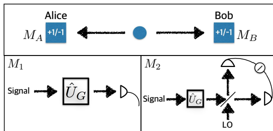
FIG. 1. Schemes for testing single-photon quantum nonlocality using feasible measurement setups. M_A ( M_B ) denote possible measurement settings of Alice (Bob), and +1/-1 denote their measurement outcomes. M_{A,B} can be either an on-off ( M_1 ) or a homodyne detection ( M_2 ), assisted by Gaussian-operations. \hat{U}_G denotes a Gaussian operation comprised of displacement and/or squeezing, and LO denotes a local oscillator (strong laser field).
