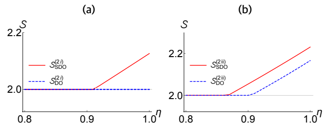
FIG. 2. Maximum values of the CHSH correlation as functions of the detection efficiency for the 2-homodyne case: (a) One party uses two Gaussian-assisted on-off detection, while the other party uses homodyne binning strategies only. (b) Each party uses both types of measurements. The solid (red) curves correspond to the squeezed-and-displaced cases, whereas the dashed (blue) curves are for the displacement-only case.
