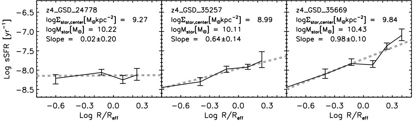
Figure 10. The sSFR as a function of radial distance to the galactic center for three z \sim 4 galaxies. The gray dotted lines are a power-law from our measurement of the sSFRs. The left panel shows a galaxy with a flat slope, indicating similar sSFRs at all radii, and in the middle and right panels galaxies have higher sSFRs far from the center, highlighting potentially reduced star-formation in their centers.
