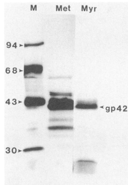
FIG. 6. Myristylation of the pre-S-S polypeptides. Sf9 cells infected with 373PS were labeled with [ ^{35}\text{S} ]methionine (Met) or [ ^3\text{H} ]myristic acid (Myr) for 4 h at 48 h postinfection and then detergent extracted. HBsAg was immunoprecipitated and examined by SDS-PAGE, fluorography, and autoradiography. The positions of molecular weight standards (M) are shown (in thousands) at the left. The pre-S-S polypeptide was efficiently labeled with both methionine and myristic acid.
