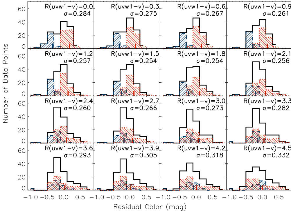
Fig. 20.— Same as Figure 19 for different choices of R_{uvw1-R_v}
