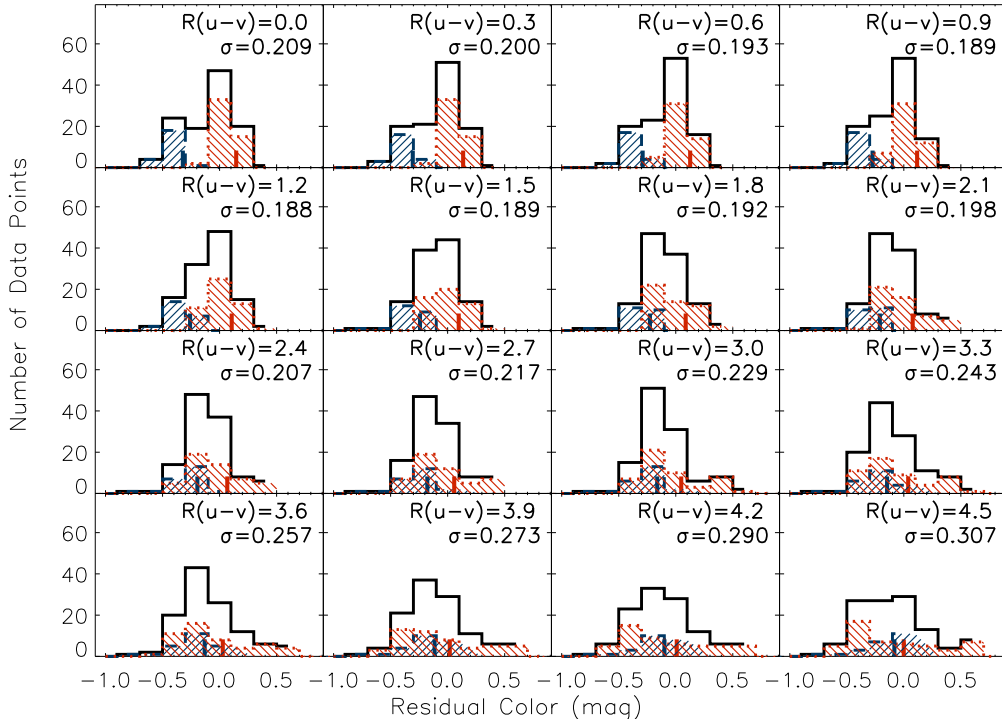
Fig. 19.— Histograms of residuals of peak-colors of SNe Ia relative to a linear function from -5 - +10 days for different choices of R_u-R_v . The slope of the color evolution is fixed, with the offset being fitted for each choice of R_u-R_v . The blue-dashed histograms show data for NUV-blue SNe, the red-dashed histograms show data for NUV-red SNe. The black-solid histogram is the combined data. Blue and red ticks show the mean residuals for NUV-blue and -red data, respectively. The scatter for the total data is shown for each choice of R_u-R_v .
