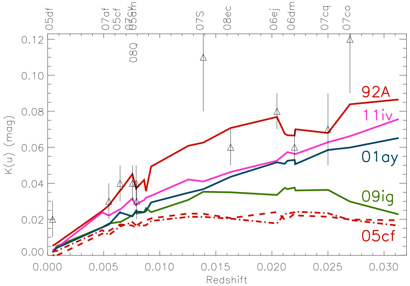
Fig. 21.— Near-peak K-corrections for the u -band based upon three spectra. NUV-red corrections are shown in red and are based on an HST/optical spectrum of SN 1992A (Kirshner et al. 1993) (solid-line) and two spectra of SN 2005cf (Wang et al. 2009a) (dashed lines). NUV-red-irregular corrections are shown in green and are based on a Swift UVOT spectrum of SN 2009ig. Narrow-peaked corrections are shown in pink and are based on an HST/optical spectrum of SN 2011iv (Foley et al. 2012b). The K -corrections presented in B10 are shown as open diamonds, and in most cases agree with the SN 1992A corrections derived in this work.
