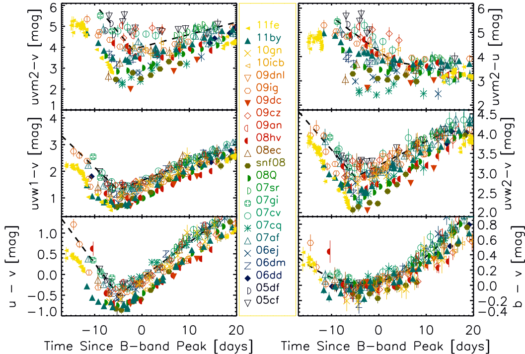
Fig. 3.— Near-peak colors of 23 normal SNe Ia compared to the v band. The “NUV-blue” group is shown with filled symbols, the “NUV-red” group with open symbols, the MUV-blue group is shown with pluses and crosses. The uvm2 - u colors are shown in the upper right panel to permit comparison of MUV versus NUV colors.
