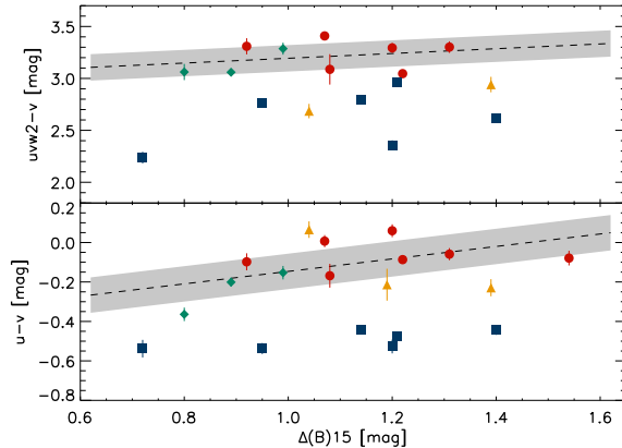
Fig. 16.— u - v colors at BPEAK plotted versus the optical peak width, \Delta m_{15}(B) . SNe Ia are grouped as NUV-blue (blue-square), NUV-red (red-circle), MUV-blue (orange-triangle) and irregular (green-diamond). Both the NUV-red and NUV-blue groups appear to span the range of peak widths. A linear peak-width, peak-color relation for the NUV-red and irregular SNe Ia is shown with 1\sigma scatter. The linear relation is: (u-v)_{BPEAK} = (0.33)\Delta m_{15}(B) - 0.54 .
