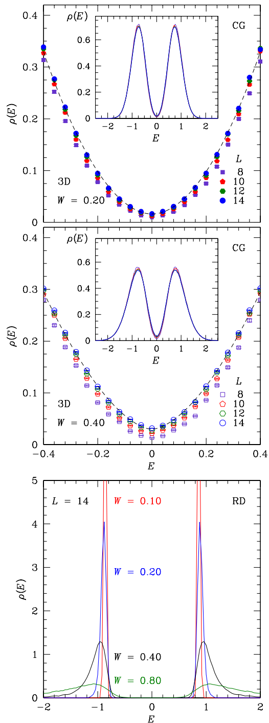
FIG. 1: (Color online) Top: DOS for the 3D CG model for W = 0.20 . The data are well fit by \rho(E) \sim |E|^\delta , \delta \approx 2 (dashed lines are a guide to the eye) around the Fermi level. Center: Same as in the top panel for W = 0.40 . The insets show the full DOS. Both panels have the same horizontal range. Bottom: DOS for the 3D RD model. For all W studied the data show a bimodal structure with peaks at |E| \sim 1 and a hard gap of size \sim 2 , in stark contrast to the CG model.
