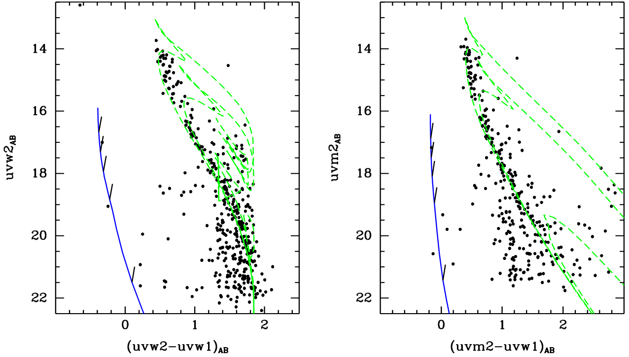
Fig. 6.— NGC 2539 color-magnitude diagrams. Isochrones from the Padova group are overlaid with parameters set to [\text{Fe}/\text{H}] = +0.0 , E(B - V) = 0.05 , (m - M)_0 = 10.65 , and ages of 630 Myr, 1 Gyr and 5 Gyr. The solid blue line is a 0.5 M_\odot white dwarf cooling curve using cooling curves and synthetic photometry from Bergeron et al. (2011).
