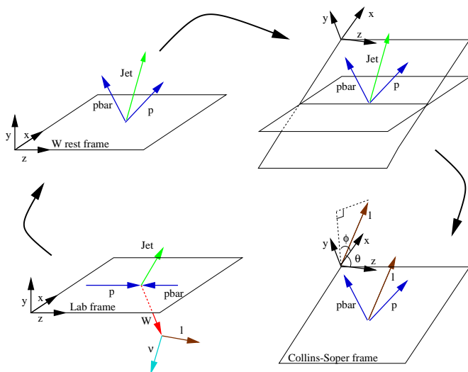
FIG. 1: Transforming from the laboratory frame to the Collins-Soper frame. We first boost to the W rest-frame, then rotate the x - z plane so that it coincides with the p - \bar{p} plane. Finally we rotate the frame around the y -axis so that the z -axis bisects the angle between \vec{p} and -\vec{p} . The positive y axis is selected to have the same direction as \vec{p}_{CS} \times \vec{l}_{CS} .
