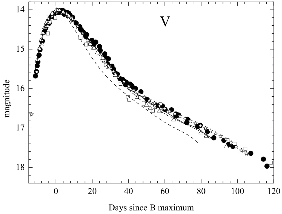
Fig. 5.— Same as Fig. 3 but for the V-band light curve.
