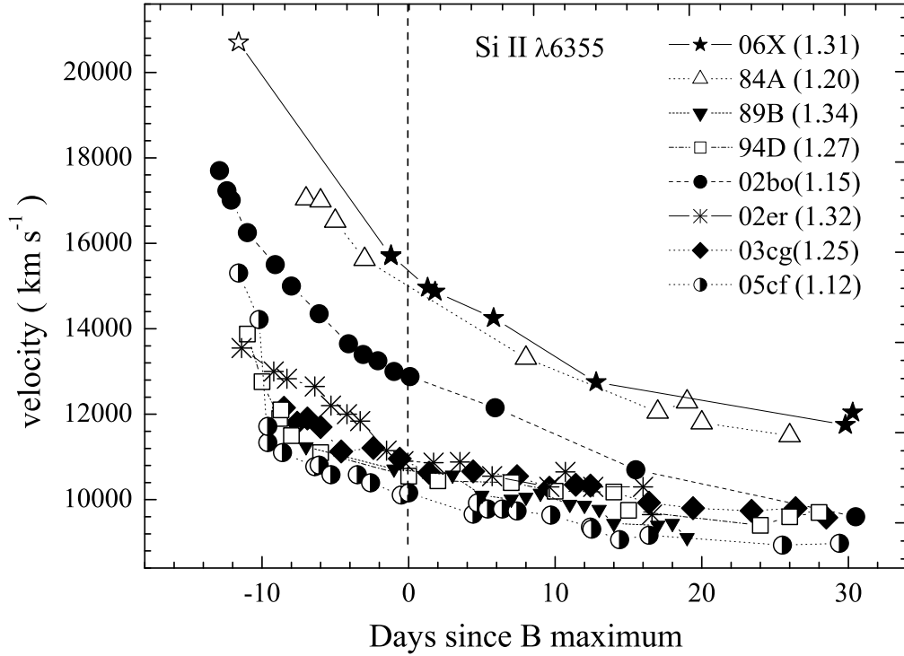
Fig. 16.— Evolution of the expansion velocity of SN 2006X as measured from the minimum of Si II \lambda 6355, compared with the values of SNe 1984A taken from Barbon et al. (1989), 1989B from Barbon et al. (1990), 2002bo from Benetti et al. (2004), 1994D from Patat et al. (1996), 2003cg from Elias-Rosa et al. (2006), 2002er from Pignata et al. (2004), and 2005cf from Garavini et al. (2007). Some of the data points in the plot are from our unpublished spectral library. The numbers in parentheses represent the \Delta m_{15} values for the SNe Ia.
