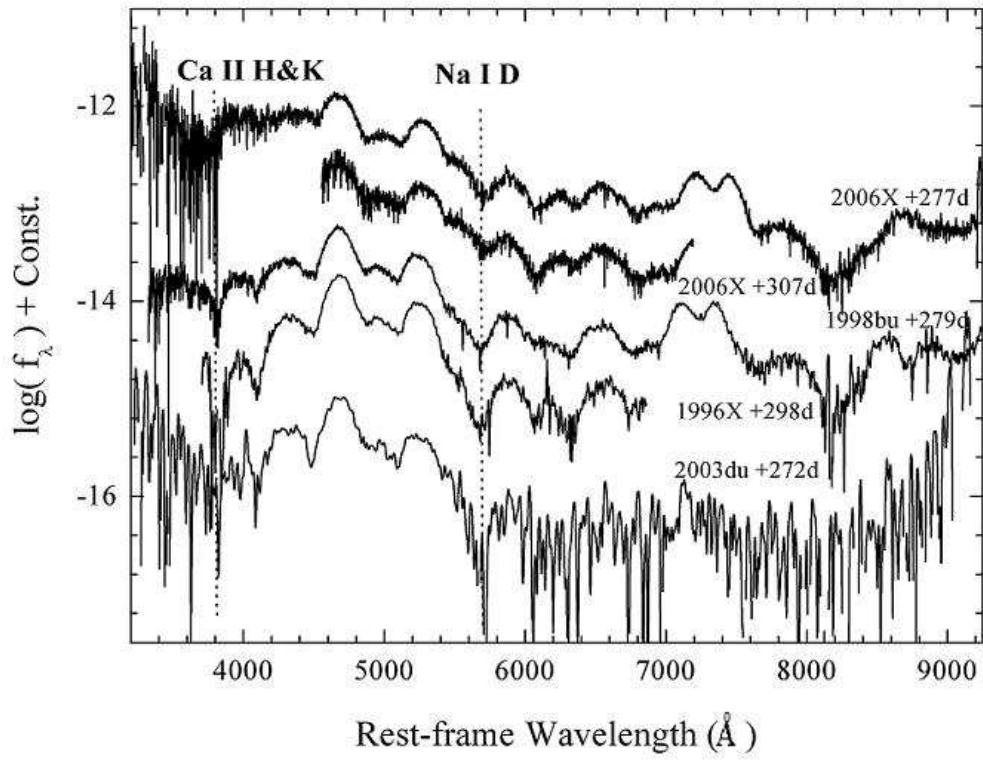
Fig. 19.— Very late-time nebular spectrum of SN 2006X compared with those of SNe 1996X, 1998bu, and 2003du. The two vertical dotted lines refer to the Ca II \lambda 3945 and Na I \lambda 5892 absorptions.
