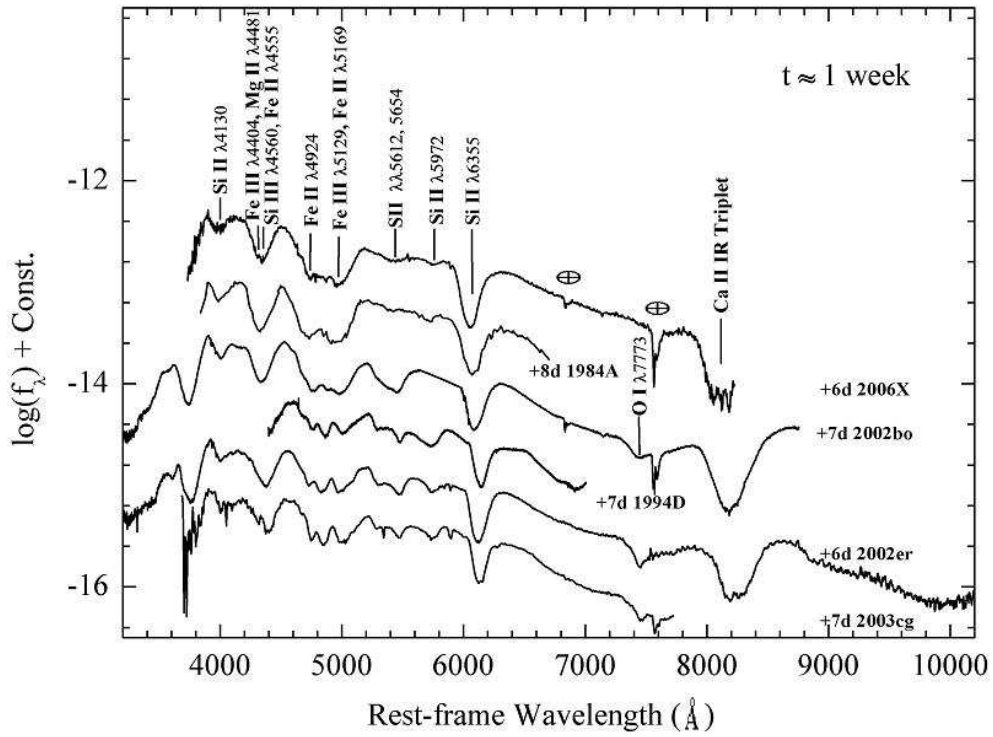
Fig. 14.— Same as Fig. 13 but for spectra about one week after B maximum.
