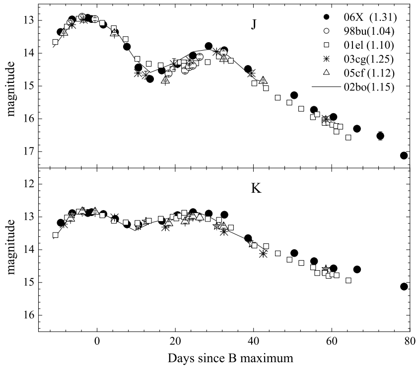
Fig. 8.— Near-IR J -band and K -band light curves of SN 2006X compared with those of SNe 1998bu, 2001el, 2002bo, 2003cg, and 2005cf. The data sources are cited in the text.
