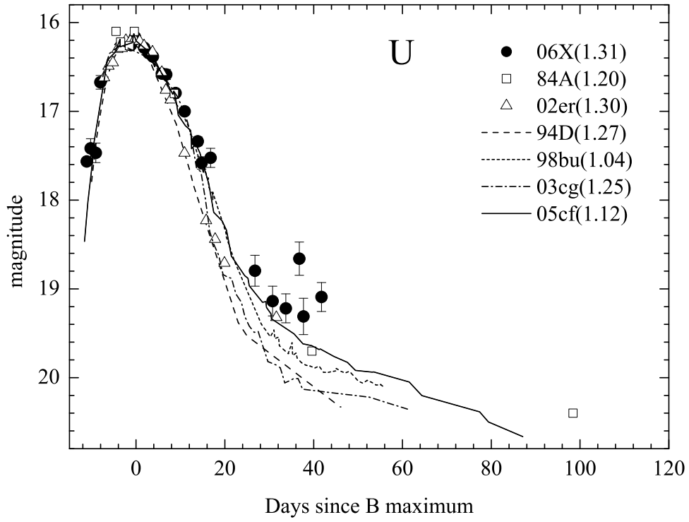
Fig. 3.— Comparison of the observed U -band light curves of SN 2006X with those of SNe 1984A, 1994D, 1998bu, 2002er, 2003cg, and 2005cf. All light curves are arbitrarily shifted in time and magnitude to fit the peak value of SN 2006X. The data sources are cited in the text.
