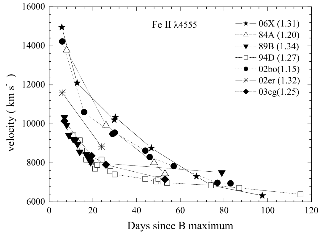
Fig. 17.— The same as Fig. 16, but for the Fe II \lambda 4555 line.
