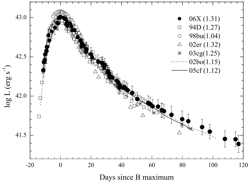
Fig. 20.— The quasi-bolometric light curve of SN 2006X computed from the UBVR IJK light curves. Error bars consist of the uncertainties in the photometry, the distance and absorption corrections. The quasi-bolometric light curves constructed from SNe 1994D, 1998bu, 2002bo, 2002er, 2003cg, and 2005cf are overplotted for comparison (see §3.1 for the data sources). The numbers in parentheses represent the \Delta m_{15} values for the SNe Ia.
