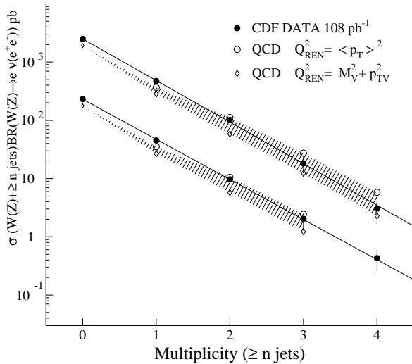
FIG. 1. Cross sections for W^\pm \rightarrow e^\pm \nu + \geq n jets (top) and Z \rightarrow e^+ e^- + \geq n jets (bottom) versus inclusive jet multiplicity. The lines are fits to an exponential to the data. The theory is shown as a shaded band which represents the uncertainty due to the renormalization scale. The \geq 0 jet prediction is a Born-level calculation for W production.
