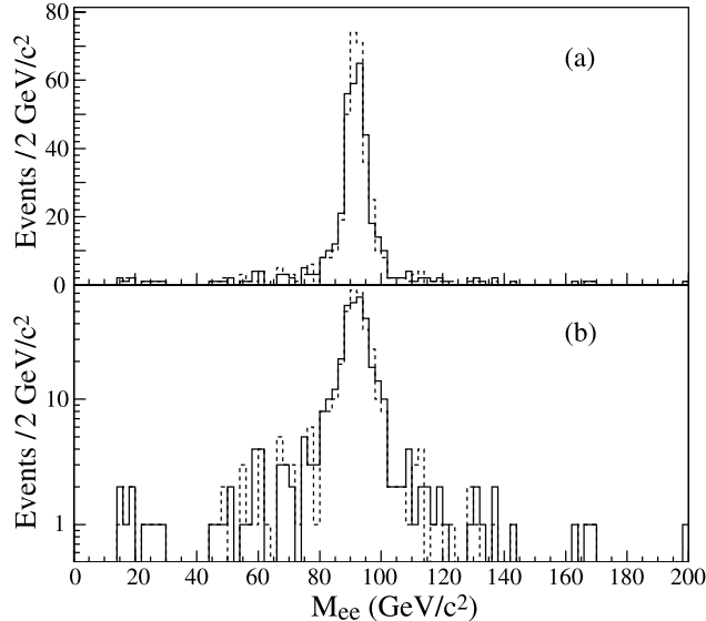
FIG. 1: Z(\rightarrow ee) + 2j data before (solid) and after (dashed) revertexting: (a) has a linear scale and illustrates the improvement in the Z -boson mass resolution after the revertexting; (b) has a logarithmic scale and shows the suppression of the background from vertex misidentification in the tails of the Z -boson peak.
