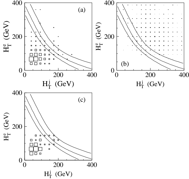
FIG. 5: H_T^e versus H_T^j for (a) the predicted background, (b) 200 GeV/ c^2 leptiquark events, and (c) the base data sample. The curved lines correspond to \mathcal{D}_{\text{NN}} = 0.5, 0.8, and 0.95 (from left to right). The area of a displayed square is proportional to the number of events in that bin, with the total number of events normalized to 123 \text{ pb}^{-1} .
