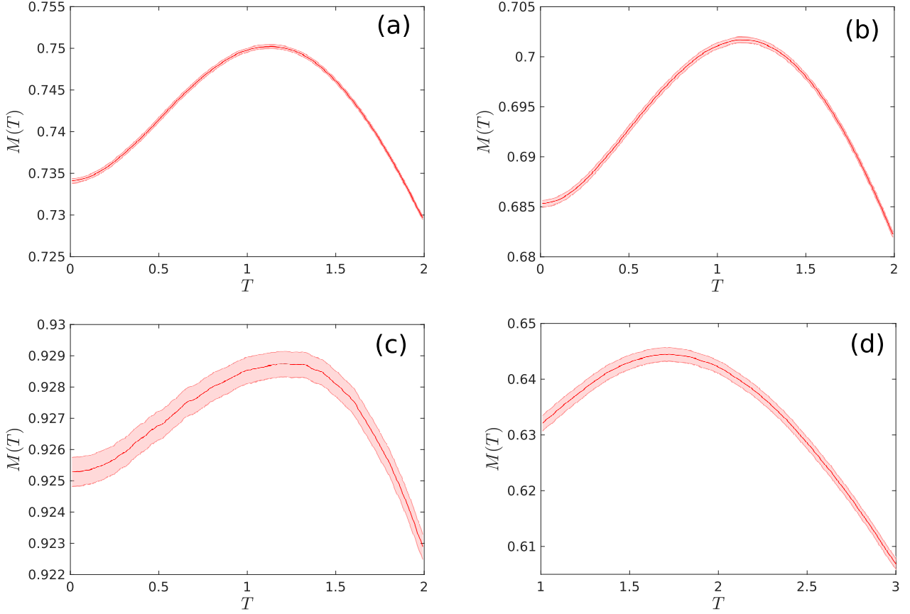
FIG. 3: (Color online) Mean of the overlap M(T) and its standard deviation as functions of the temperature T : data for the ladder (a) for \sigma = 1 and \gamma = 0.5 and (b) for \sigma = 2 and \gamma = 0.4 ; data for the stacked ladder (c) for \sigma = 1 and \gamma = 0.5 and (d) for \sigma = 2 and \gamma = 0.4 .
