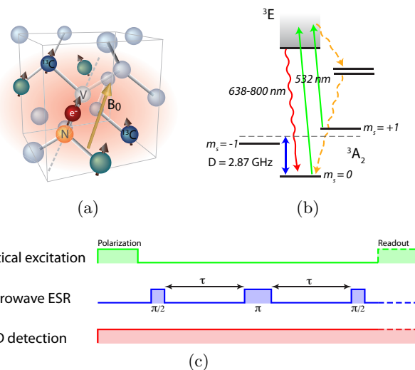
FIG. 1: (a) NV electronic spin axis is defined by nitrogen and vacancy sites, in one of four crystallographic directions. NV orientation subsets in an ensemble can be spectrally selected by applying a static magnetic field, B_0 . Also shown are ^{13}\text{C} nuclear spins and other paramagnetic impurities such as substitutional nitrogen. (b) NV center electronic energy level structure. Spin polarization and readout is performed by optical excitation and fluorescence detection. Ground state spin manipulation is achieved by resonant microwave excitation. The ground state triplet has a zero magnetic field splitting D \simeq 2.87 \text{ GHz} . (c) Hahn-echo experimental sequence used in present measurements.
