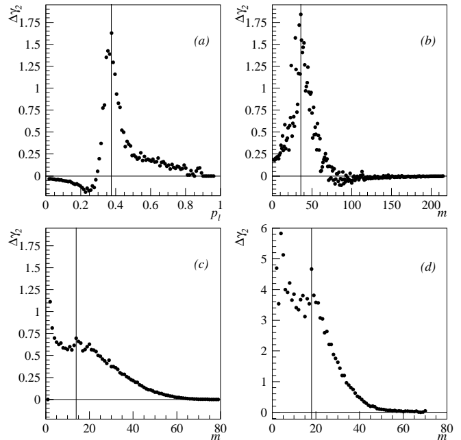
FIG. 4. The quantity \Delta\gamma_2 for: (a) percolation ( A_0 = 216 ) as a function of p_l , (b) percolation as a function of m , (c) random partitions as a function of m and (d) Au + C multifragmentation as a function of m . Solid vertical lines indicate the guess for the critical point.
