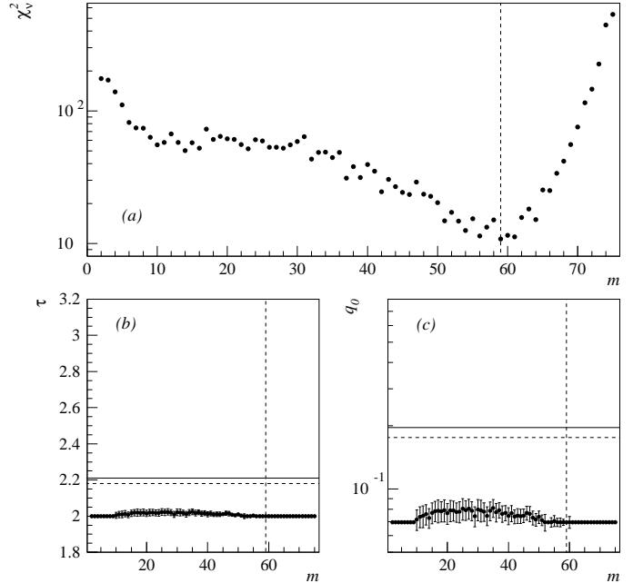
FIG. 14. Results for the full Fisher \tau -power law analysis on random partitions: (a) \chi_\nu^2 , (b) fitted \tau and (c) q_0 . The horizontal solid (dashed) lines show the accepted values of \tau and q_0 for percolation (3D Ising).
