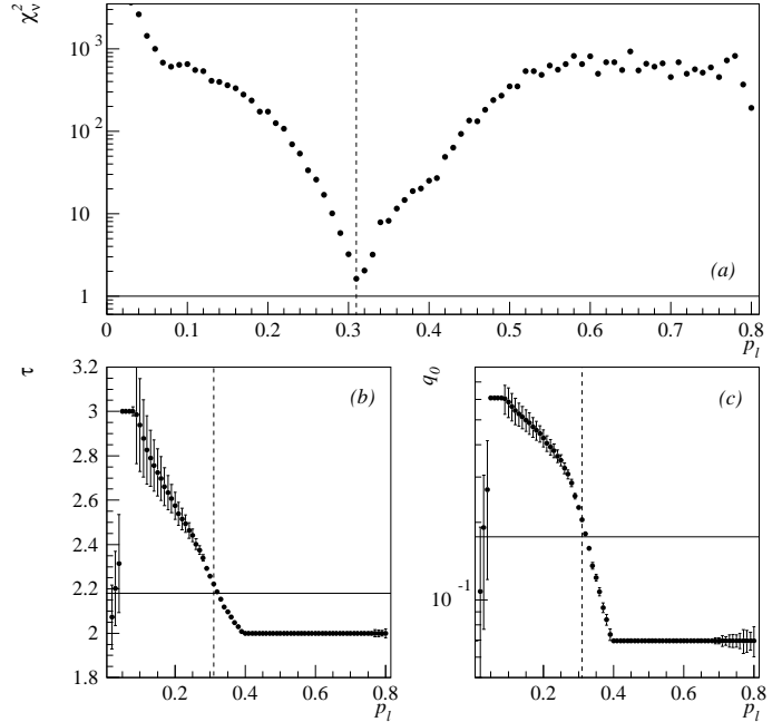
FIG. 12. Results for the full Fisher \tau -power law analysis on percolation as a function of p_l : (a) \chi_\nu^2 , (b) fitted \tau and (c) q_0 . The vertical dashed line shows the estimate of the critical point based on a best fit based on \chi_\nu^2 . The horizontal solid lines show the accepted values of \tau and q_0 for percolation.
