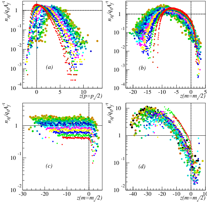
FIG. 20. Results of the scaling function analysis with the critical point equal to half the value as determined from the Fisher \tau -power law analysis for: (a) percolation as a function of z(p_l) , (b) percolation as a function of z(m) , (c) random partitions as a function of z(m) and (d) Au + C multifragmentation as a function of z(m) .
