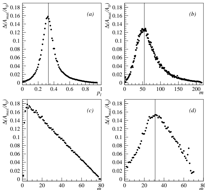
FIG. 1. Fluctuations in the normalized size of the largest cluster for: (a) percolation ( A_0 = 216 ) as a function of p_l , (b) percolation as a function of m , (c) random partitions as a function of m and (d) Au + C multifragmentation as a function of m . Solid vertical lines indicate the guess for the critical point.
