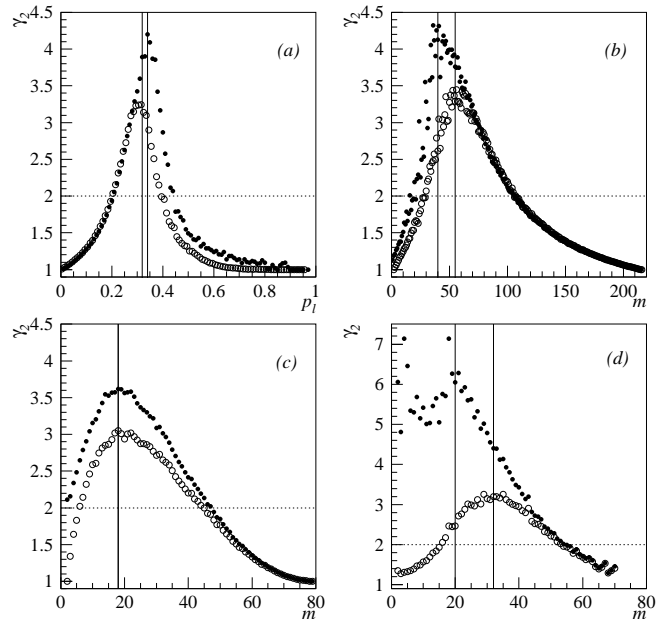
FIG. 2. Fluctuations as measured by \gamma_2 for: (a) percolation as a function of p_l , (b) percolation as a function of m , (c) random partitions as a function of m and (d) Au + C multifragmentation as a function of m (at low m \overline{\gamma}_2 is affected by fission events not completely filtered). Open circles show \langle \gamma_2 \rangle , while filled circles show \overline{\gamma}_2 (see text for details). Solid vertical lines indicate the guess for the critical point. A dotted horizontal line shows the value of \gamma_2 = 2 .
