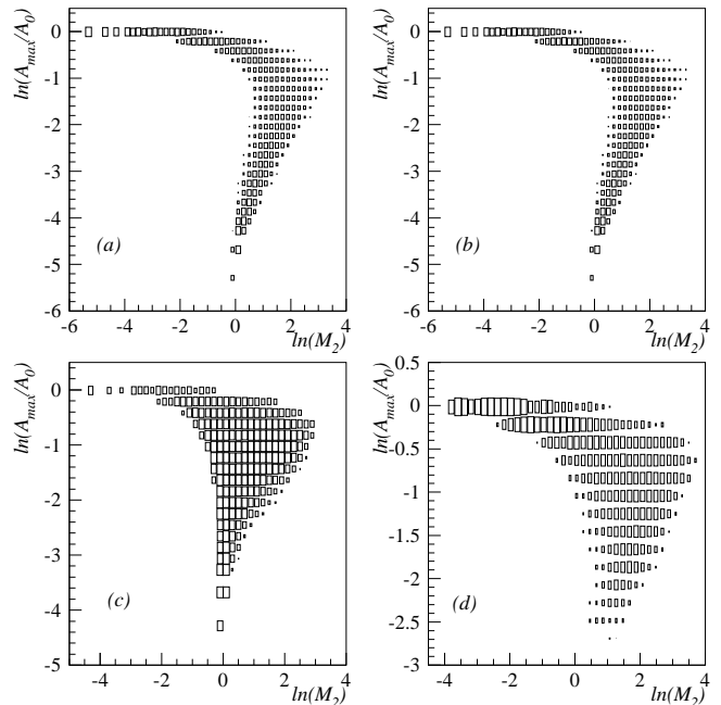
FIG. 6. Campi plots of the cluster distributions for: (a) percolation as a function of p_l , (b) percolation as a function of m , (c) random partitions as a function of m and (d) Au + C multifragmentation as a function of m .
