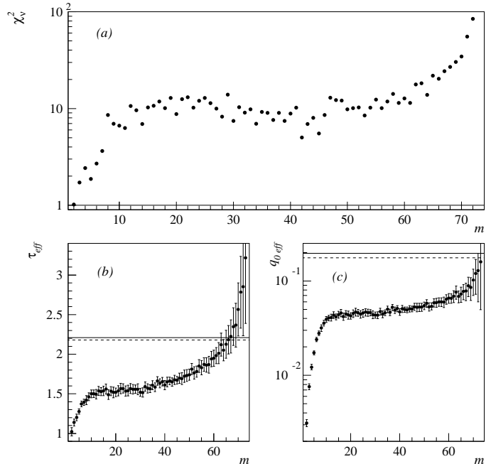
FIG. 10. Results for \tau_{eff} -minimum analysis on random partitions: (a) \chi_v^2 , (b) fitted \tau_{eff} and (c) q_0 . The horizontal solid (dashed) lines show the accepted values of \tau and q_0 for percolation (3D Ising).
