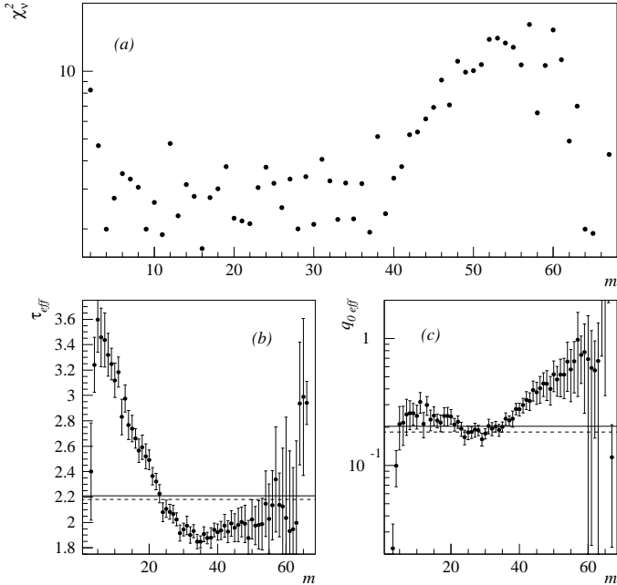
FIG. 11. Results for \tau_{eff} -minimum analysis on Au + C multifragmentation: (a) \chi_\nu^2 , (b) fitted \tau_{eff} and (c) q_0 . The horizontal solid (dashed) lines show the accepted values of \tau and q_0 for percolation (3D Ising).
