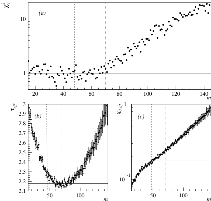
FIG. 9. Results for \tau_{eff} -minimum analysis on percolation as a function of m : (a) \chi_v^2 , (b) fitted \tau_{eff} and (c) q_0 . The vertical dotted line show the location of the minimum in \tau_{eff} . The vertical dashed line shows one instance of a better fit based on \chi_v^2 . The horizontal solid lines show the accepted values of \tau and q_0 for percolation.
