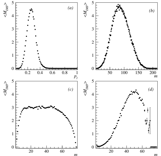
FIG. 7. Average number of intermediate mass clusters, \langle M_{IMF} \rangle , for: (a) percolation as a function of p_l , (b) percolation as a function of m , (c) random partitions as a function of m and (d) Au + C multifragmentation as a function of m .
