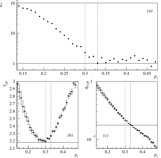
FIG. 8. Results for \tau_{eff} -minimum analysis on percolation as a function of p_l : (a) \chi_\nu^2 , (b) fitted \tau_{eff} and (c) q_0 . The vertical dotted line show the location of the minimum in \tau_{eff} . The vertical dashed line shows one instance of a better fit based on \chi_\nu^2 . The horizontal solid lines show the accepted values of \tau and q_0 for percolation.
