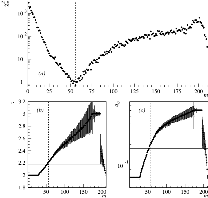
FIG. 13. Results for the full Fisher \tau -power law analysis on percolation as a function of m : (a) \chi_\nu^2 , (b) fitted \tau and (c) q_0 . The vertical dashed line shows the estimate of the critical point based on a best fit based on \chi_\nu^2 . The horizontal solid lines show the accepted values of \tau and q_0 for percolation.
