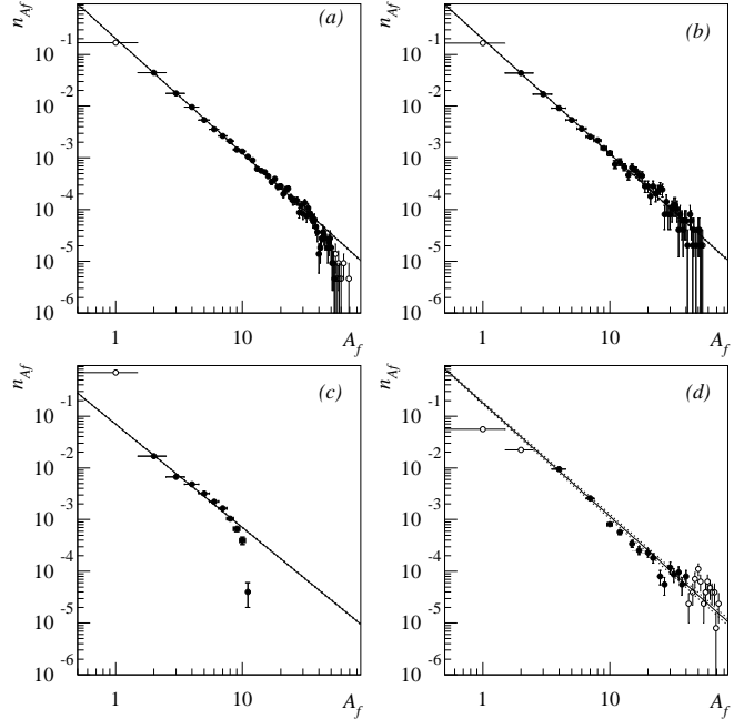
FIG. 16. Best fit Fisher \tau -power laws for: (a) percolation ( pi ), (b) percolation ( m ), (c) random partitions and (d) Au + C multifragmentation. Solid circles were included in the fits, open circles were excluded. Solid lines show the best fit power law, dotted lines indicate error in the power law based on errors in the fitted parameters.
