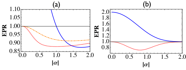
FIG. 2: Second-order EPR correlation of the non-Gaussian entangled state Eq. (2.1) as a function of |\alpha| . (a) |\psi\rangle_A = \hat{a}^\dagger|\alpha\rangle : n+m=0 (blue solid), 1 (red dotted), and 2 (orange dashed), (b) |\psi\rangle_A = |\alpha\rangle - |-\alpha\rangle : n+m = \text{even} (blue solid), and odd (red dotted)
