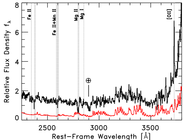
Figure 3. Composite one-dimensional IMACS spectra as a function of rest-frame wavelength for the seven galaxies within r < 1.4 Mpc of the astrometric center of ClG J0218.3-0510 with spectroscopic redshifts 1.620 \leq z \leq 1.630 (see Table 1). The black line shows the composite, weight-averaged spectrum, and the red line is the weighted uncertainty, dominated by emission from the sky. Strong [\text{O II}] is observed, as well as several absorption features, including the doublet \text{Mg II } \lambda\lambda 2976, 2804 , and absorption from blends of \text{Fe II} line. The absorption feature at rest-frame 2900 \text{ \AA} corresponds to telluric absorption at \approx 7600 \text{ \AA} in the observed frame.
