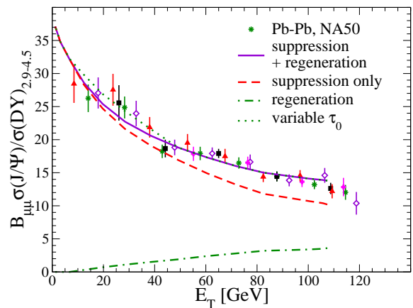
FIG. 2: Centrality dependence of J/\psi /Drell-Yan dimuons at SPS; NA50 data [31] are compared to our results with (solid line) and without (dashed line) charmonium regeneration (represented by the dot-dashed line). The dotted line includes longer thermalization times \tau_0 in peripheral collisions.
