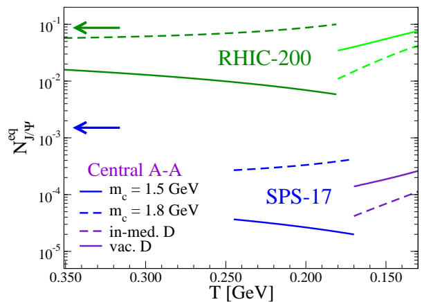
FIG. 1: Equilibrium J/\psi abundances (with m_\psi(T) \equiv m_\psi^{vac} ) in an isotropic, adiabatically expanding system at fixed N_{c\bar{c}} for SPS and RHIC conditions for two values of the charm-quark mass above T_c , and for free and in-medium charmed hadron masses below T_c .
