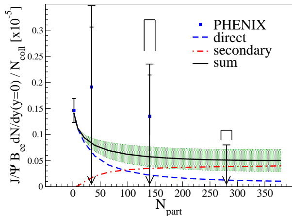
FIG. 4: J/\psi yield per binary N - N collision versus participant number in \sqrt{s_{NN}}=200 GeV Au - Au collisions. Preliminary PHENIX data [36] are compared to our model calculations; dot-dashed line: thermal regeneration; dashed line: suppressed primordial production; band: total J/\psi yields with different values for in-medium open-charm masses.
