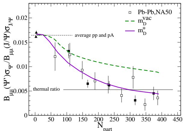
FIG. 3: Centrality dependence of the \psi'/\psi data [34] at SPS compared to our results with (full line) and without (dashed line) in-medium reduced D -meson masses.
