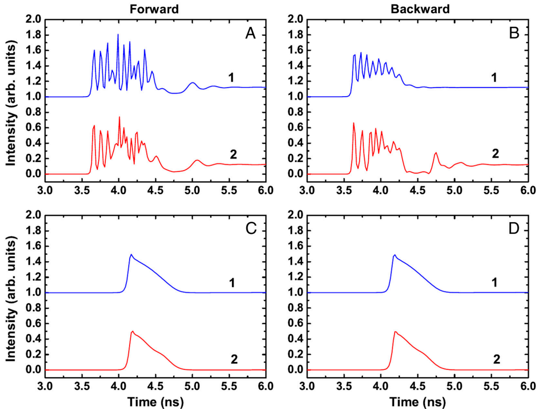
Fig. 5. Simulated forward ( A ) and backward ( B ) signals with a dephasing rate of \gamma_{\text{col}} = 1 \times 10^{10} \text{ s}^{-1} ; forward ( C ) and backward ( D ) signals with artificially large collisional dephasing ( \gamma_{\text{col}} = 1 \times 10^{11} \text{ s}^{-1} ). Curves 1 (blue) are obtained using a smooth pump pulse as the initial input, while 2 (red) used a pump pulse with random intensity fluctuations to mimic the experiment. The curves are vertically shifted for convenience.
