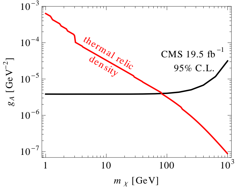
FIG. 2: Black curve gives the upper bound on the anapole moment, g_A , from CMS monojet data for the indicated anapole dark matter mass, m_\chi . Red curve gives the value of g_A needed to produce the observed dark matter abundance as a function of m_\chi .
