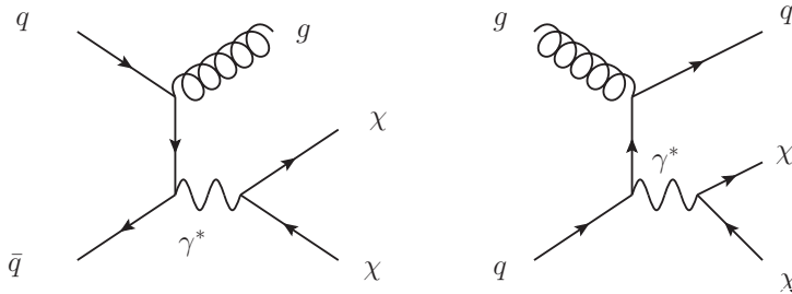
FIG. 1: Monojet diagrams at colliders. Diagrams with permuted initial particles also contribute.
