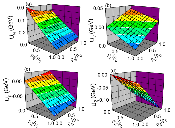
FIG. 1: (Color online) Mean-field potentials of N (a), K (c), and \bar{K} (d) at zero momentum as functions of baryon and antibaryon densities and of \pi^- (b) as a function of neutron-like and proton-like densities.
