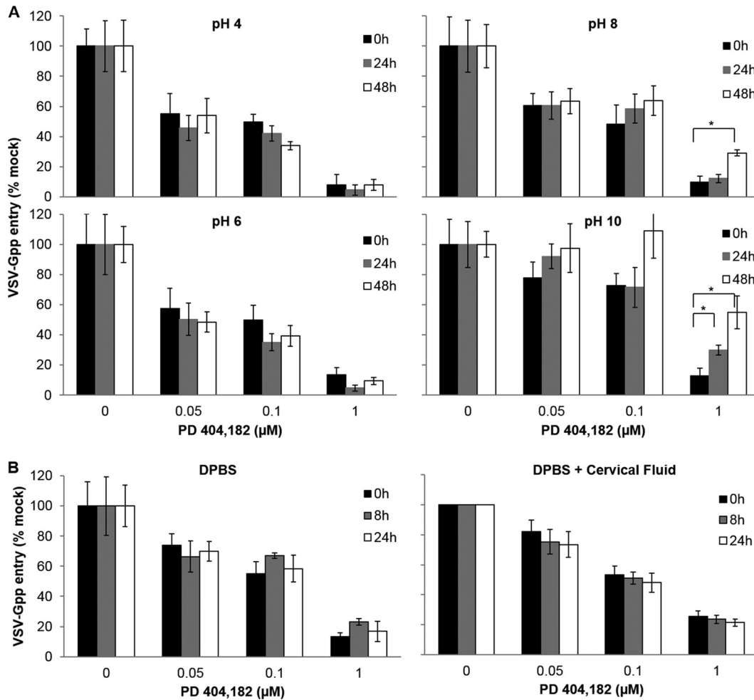
FIG 2 PD is stable and fully active at acidic pH and in cervical fluid. PD (30 \mu\text{M} ) or DMSO (10%) was incubated at 37°C for 0, 8, 24, or 48 h in DPBS adjusted to pH 4, 6, 8, or 10 (A) or 20% cervical fluid (the diluent was DPBS) (B). These PD samples were then diluted to the desired concentration in complete growth medium containing VSV-Gpp (viral supernatant diluted 500-fold), and the PD-virus mixtures were incubated at 37°C for 30 min and used to inoculate naive Huh-7.5 or 293T cells at 4°C for 2 h prior to incubation at 37°C in 5% \text{CO}_2 . The infectivity (virus entry into cells) was quantified by measuring the supernatant luciferase reporter activity at 48 h postinfection. Values and error bars represent the means and standard deviations, respectively, of at least two independent experiments carried out in duplicate. Statistical significance was determined by Student's t test (*, P < 0.01 ).
