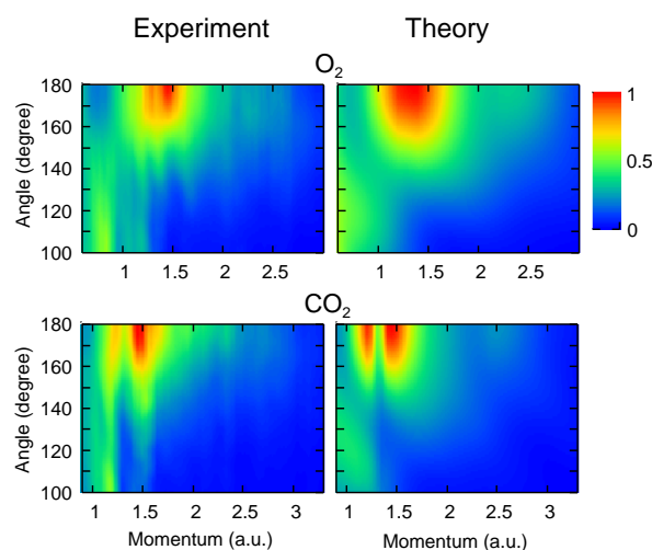
Figure 1. Experimental and theoretical elastic DCSs for scattering of free electrons from partially aligned O_2^+ and CO_2^+ . The theoretical results were obtained by a convolution with MO-ADK angle-dependent ionization rates.
