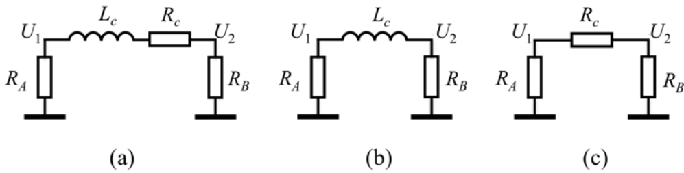
Figure 2. Lumped impedance-components-based model of a short cable at low frequencies for analyzing voltage drop along the cable and phase shift in the quasi static limit [2]. Part (a) represents a cable with loss (cable inductance and resistance are designated L_c and R_c , respectively), and part (b) represents a lossless cable. Part (c) is used to determine the voltage drop in the asymptotic case where loss dominates the cable impedance (this case is not practical and is used only for the sake of analysis).
