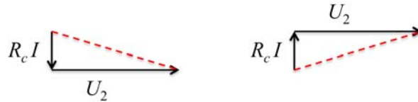
Figure 4. Illustration showing that added orthogonal noise voltages produce the same RMS voltage and mean-square voltage even if the sign of the current is flipped to the opposite value. The resulting time-dependent voltages will be different although their RMS and mean-square and RMS amplitudes remain the same.
