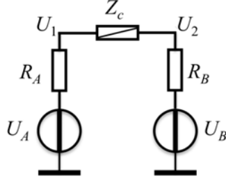
Figure 3. Circuit for impedance-based analysis of GAA's attack, as described in the main text.
