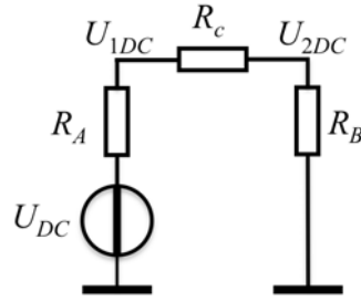
Figure 5. Schematic circuit for illustrating parasitic DC and low-frequency artifacts caused by ground loops. For the sake of simplicity, the parasitic source is assumed to exist solely at Alice's side. Only the parasitic voltage generator is shown, because its impact is additive to the voltages caused by other circuit deficiencies. The parasitic DC or low-frequency components U_{1DC} and U_{2DC} of U_1 and U_2 , respectively, are sensitive to the location of the low/high resistor at Alice's and Bob's side.
