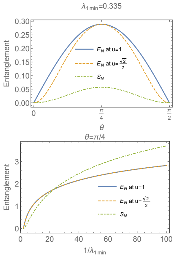
FIG. 4: (Color online). Output entanglement from mixing a nonclassical state with a vacuum at a BS quantified by two measures of degree of entanglement. (a) For constant nonclassicality, the relation of the degree of entanglement vs \theta for different purities of the input nonclassical state. (b) At optimal BS angle, the monotonic relation of the degree of entanglement vs the inverse of the minimum eigenvalue.
