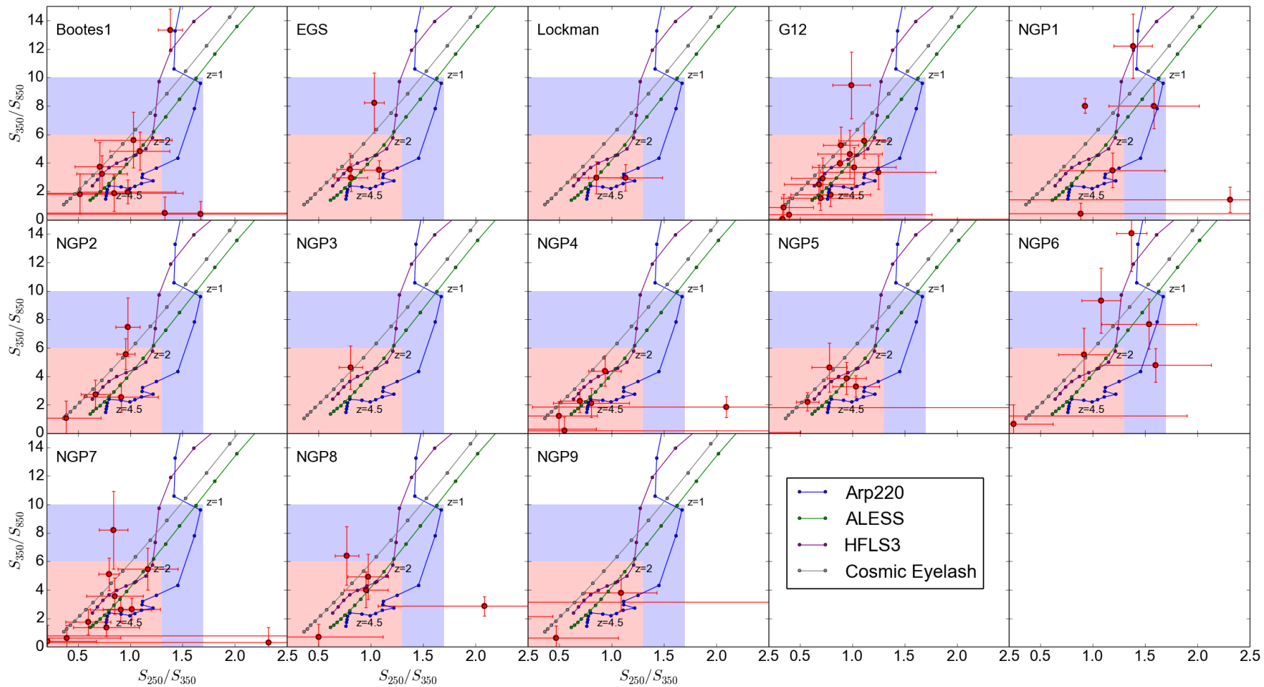
Figure 3. Submillimetre colour-colour plots, specifically 250\mu\text{m}/350\mu\text{m} versus 350\mu\text{m}/850\mu\text{m} plots of 13 candidate protocluster fields observed with SCUBA-2 in this paper. Red points and error bars represent the 850\text{-}\mu\text{m} sources in the candidate protocluster fields. Errors are propagated from the 250\text{-} , 350\text{-} , and 850\text{-}\mu\text{m} flux densities of individual sources. Blue, green, purple and grey curves are the redshift tracks on this colour-colour plot from z=0.0 to 4.5 with 0.25 steps, using templates of Arp220, ALESS, HFLS3 and Cosmic Eyelash, respectively. Based on the redshift tracks of the template SEDs, we identify colours where sources are potentially at z \geq 2 as the red region, and colours where sources are potentially at 1 < z < 2 as the blue region.
