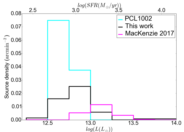
Figure 7. Distribution of infrared luminosity ( L_{\text{IR}} ) of sources in our 13 candidate protoclusters (black), a known DSFG-rich protocluster at z \sim 2 , PCL1002 (cyan), and sources in candidate protoclusters in MacKenzie et al. (2017) (magenta). SFRs are also shown in the upper horizontal axis following a linear relation with the L_{\text{IR}} (Kennicutt 1998).
