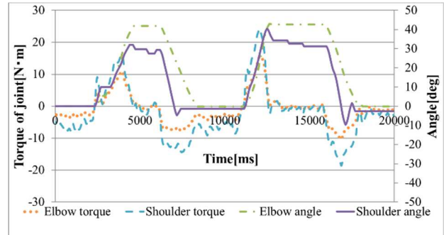
Fig. 7 Exoskeleton's data of power assisting experiment
