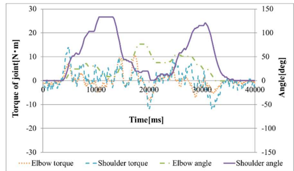
Fig. 5 Results of detecting motion intention
