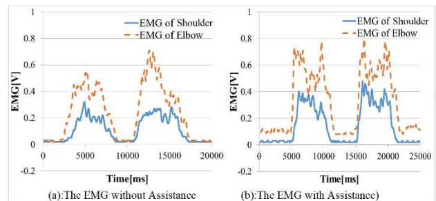
Fig. 8 Experiment evaluation using myoelectric signals
