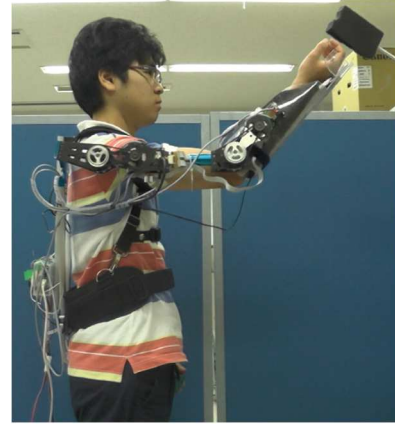
Fig. 4 Verification experiment to detect motion intention
