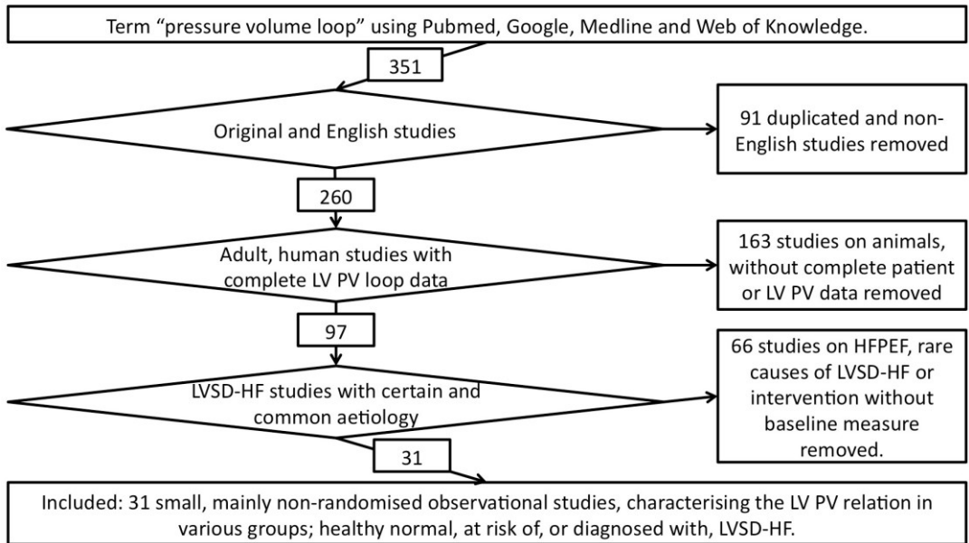
Figure 2. Flow diagram demonstrating inclusion and exclusion criteria for left ventricular pressure-volume loop studies. HFPEF 5 heart failure with preserved ejection fraction, LV 5 left ventricle, LVSD 5 left ventricular systolic dysfunction, PV 5 pressure volume,
