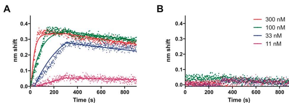
Figure 4. Biolayer interferometry analysis of TTHA0973 binding to DNA. Shown are raw traces (dots) and best-fit lines of TTHA0973 binding to (A) ST2_0973_R5_wt consensus DNA or (B) ST2_REPSA control DNA. TTHA0973 concentrations investigated include 300 nM (red), 100 nM (green), 33 nM (blue), and 11 nM (magenta).
