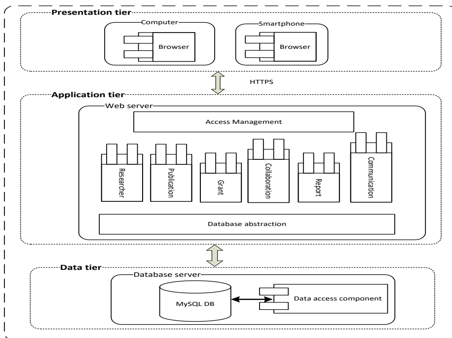
Figure 4. Client-Server architecture of RAMS
