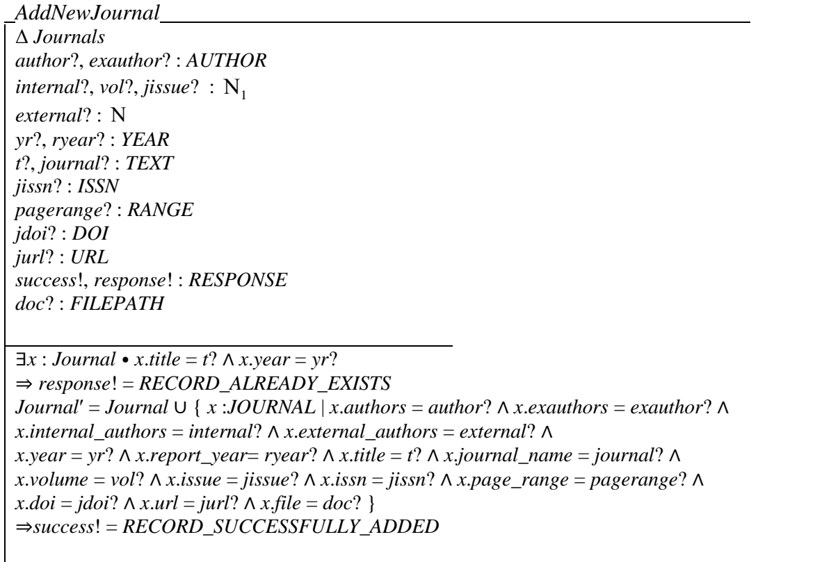
Figure 2. Z schema for adding a journal into the system
