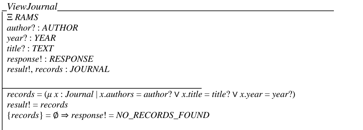
Figure 3. Z schema for viewing journal articles
