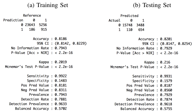
Fig. 10: Confusion Matrices and Statistics for RF
