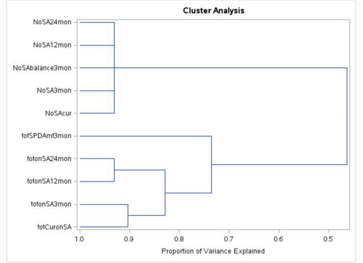
Fig. 7: Performance of Variable Clustering among 10 service variables
