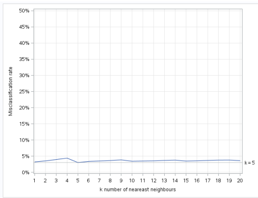
Fig. 8: Misclassification rates for the testing dataset ( k is from 1 to 20)
