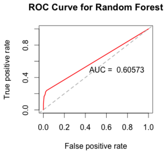
Fig. 11: ROC Index and AUC Index for RF
