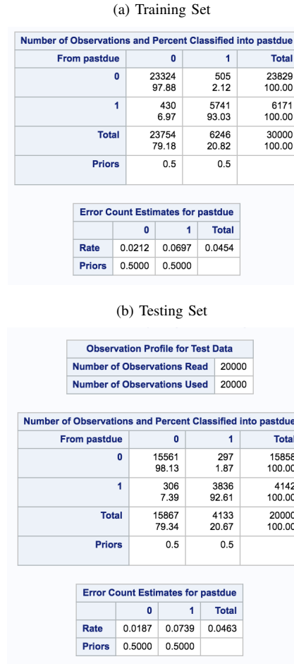
Fig. 9: Classification Summary Using 5 Nearest Neighbors
