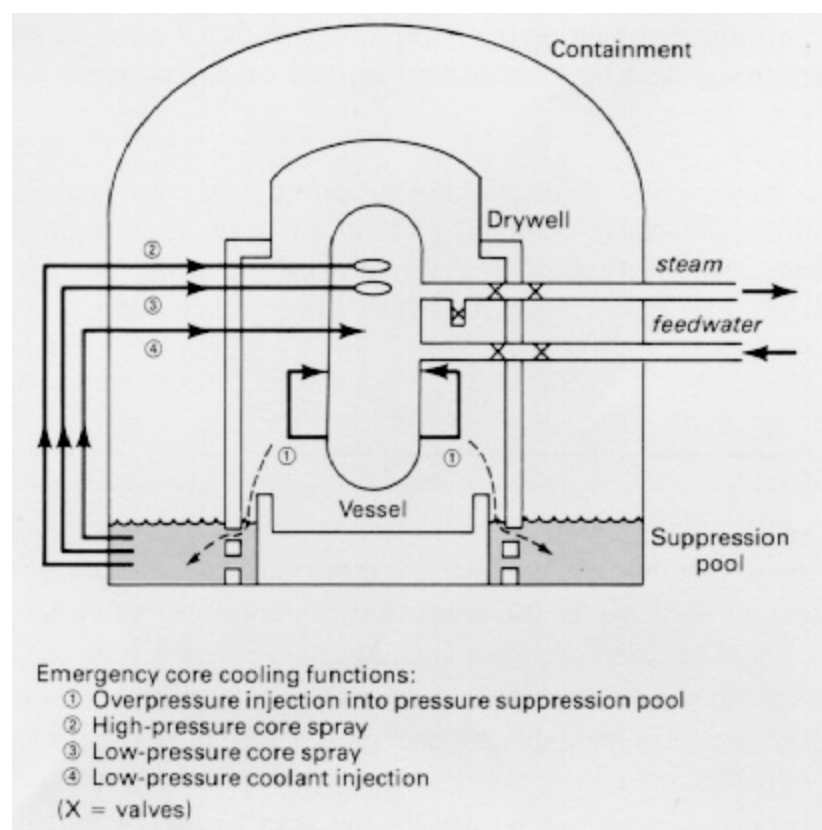
Figure 6. BWR emergency core cooling systems
