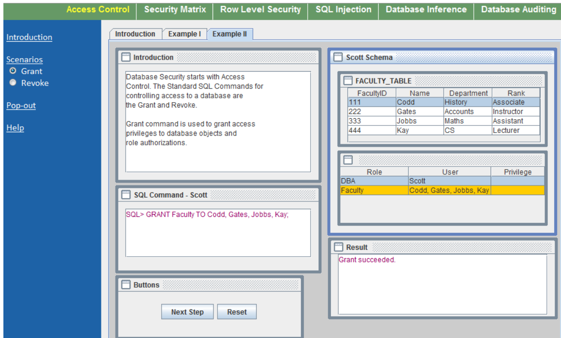
Figure 1. ADbC Access Control Sub-module: Example Granting Role Authorization
