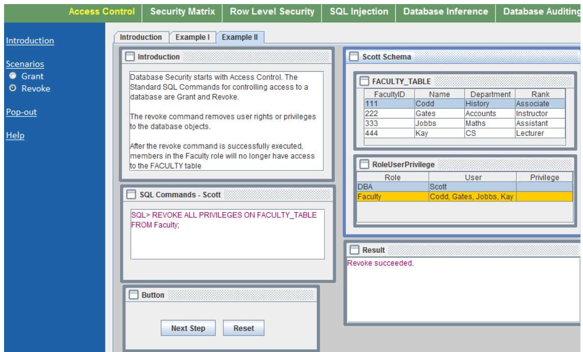
Figure 2. ADbC Access Control Sub-module: Example Revoking Role-based Privileges
