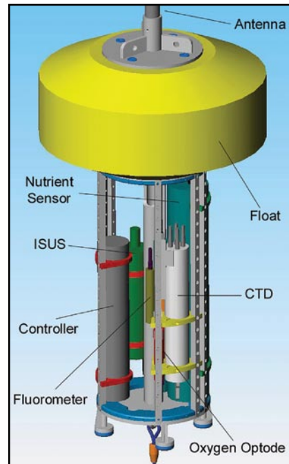
Figure 2. The instrumentation integrated into the LOBO moorings is a combination of commercially available (YSI 9600 nitrate monitor, Aanderaa oxygen optode, Sea Bird conductivity-temperature-depth sensor [CTD], fluorometer and turbidity sensors, RD Instruments acoustic Doppler current profiler) and “in house” (in situ ultraviolet spectrophotometer [ISUS]) technology. Combined with a mooring system that allows for long-term deployment and rapid data transmission through a wireless local area network, the sensors can return near-real-time information for extended deployment periods. For more detailed information on the mooring instrumentation, go to http://www.mbari.org/lobo/instruments.htm .
