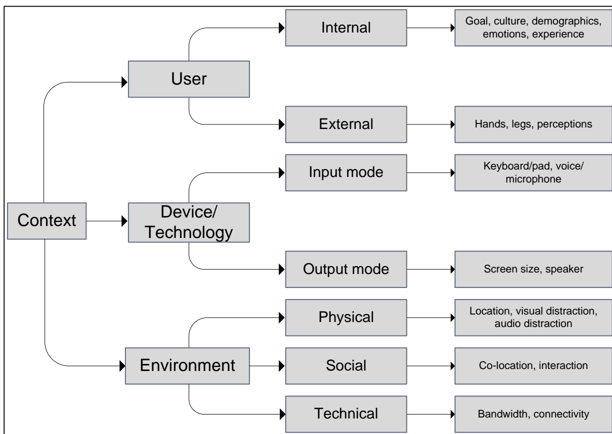
Figure 1. Context classification.
