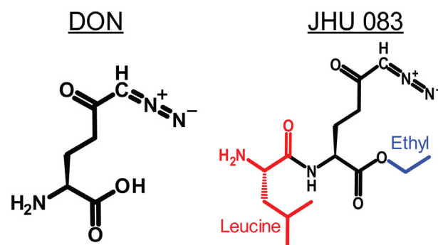
Figure 1. Chemical structure of 6-diazo-5-oxo-L-norleucine (DON) and the prodrug JHU-083 (Ethyl 2-(2-Amino-4-methylpentanamido)-DON).
