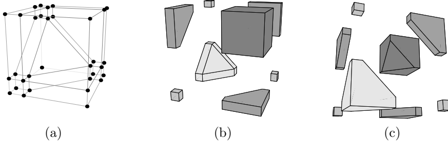
Figure 6.2: Regions where the analytic solution in 3D has constant gradient: with wire frames viewed from the positive octant (a), and exploded views of the solid regions from the positive octant (b), and the negative octant (c).
