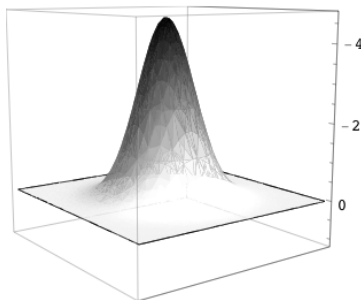
Figure 6.3: Graph of f(x_1, x_2) = -(4 + 5x_1x_2^2) e^{-30[(x_1-1/2)^2 + (x_2-1/2)^2]} , shown upside down.
