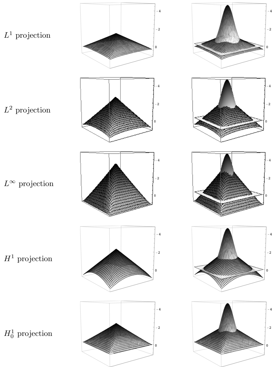
Figure 6.4: Projections and its comparisons to the function of figure 6.3, shown upside down.
