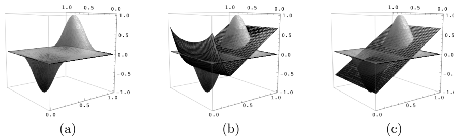
Figure 6.5: Non-uniqueness of the L^\infty projection. (a) original function, (b) and (c) two optimal solutions.
