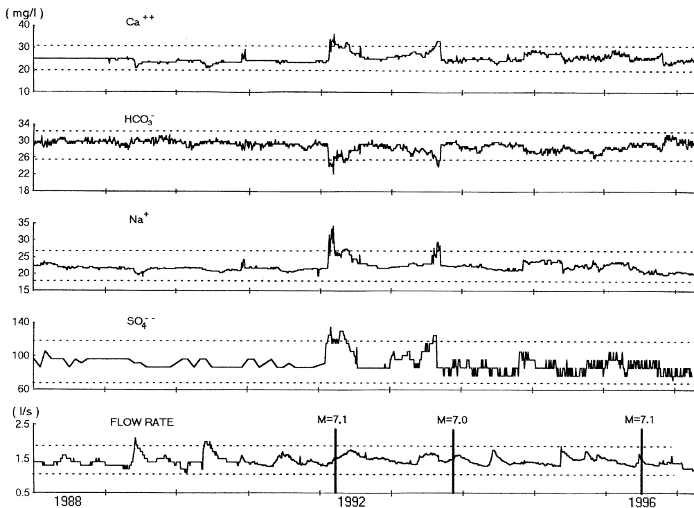
Fig. 3. – Time-series of Ca^{++} , HCO_3^- , Na^+ , SO_4^{--} contents and flow rate at the Morosnaya well. In each plot the dotted lines represent the \pm 3\sigma level. The ions contents are in mg/l; the flow rate in l/s.
