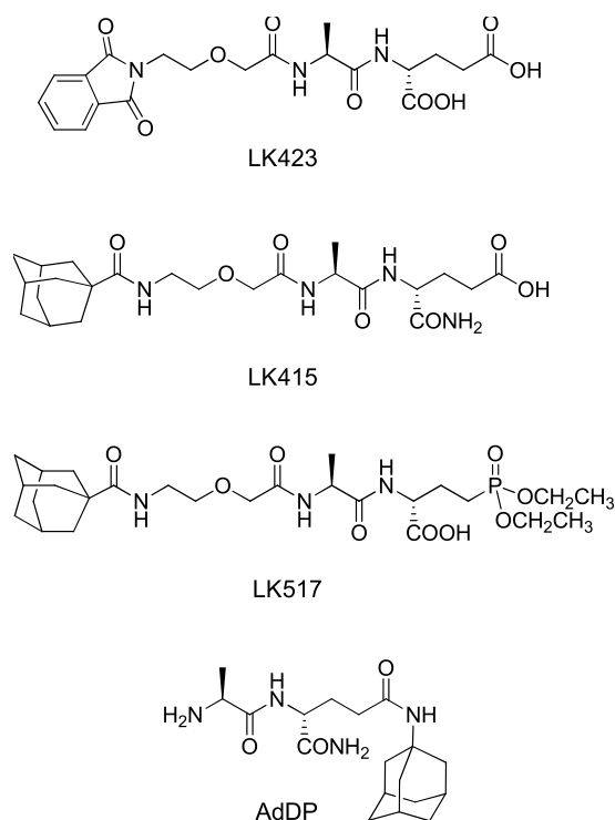
Figure 5. Phthalimido and adamantyl containing desmuramyl dipeptides.
