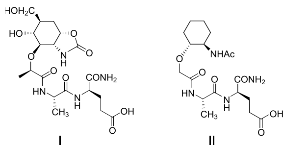
Figure 4. Carbocyclic desmuramyl peptides.
