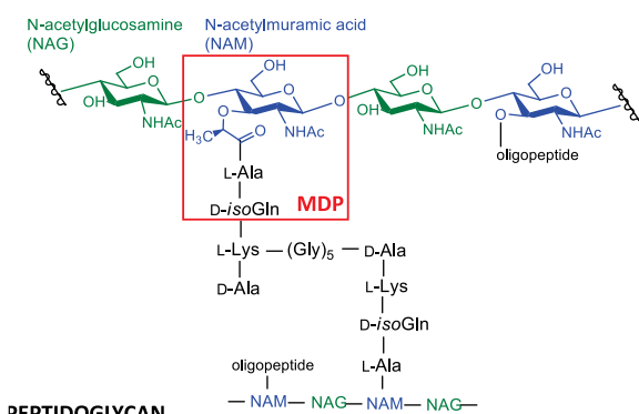
Figure 1. MDP, the smallest peptidoglycan fragments with immunostimulating properties.
