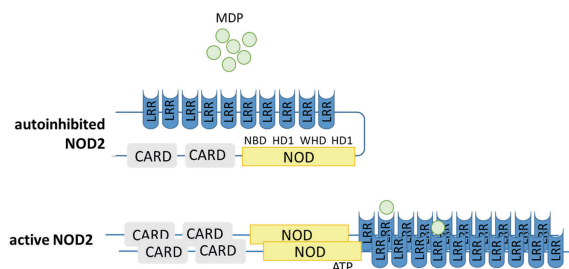
Figure 3. NOD2 changes upon MDP binding.
