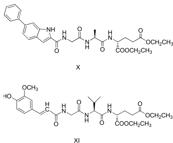
Figure 8. The most active lipophilic aryl desmuramyl peptides.
