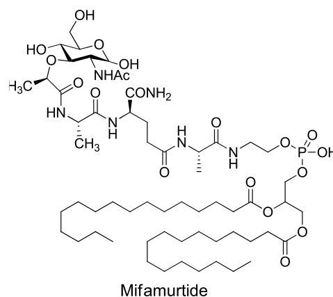
Figure 2. MDP derivatives used in clinics.
