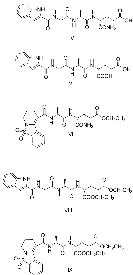
Figure 7. Indole scaffold and pyrido-fused [1,2]-benzothiazole based desmuramyl peptides.
