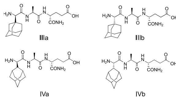
Figure 6. Adamantyl tripeptides.
