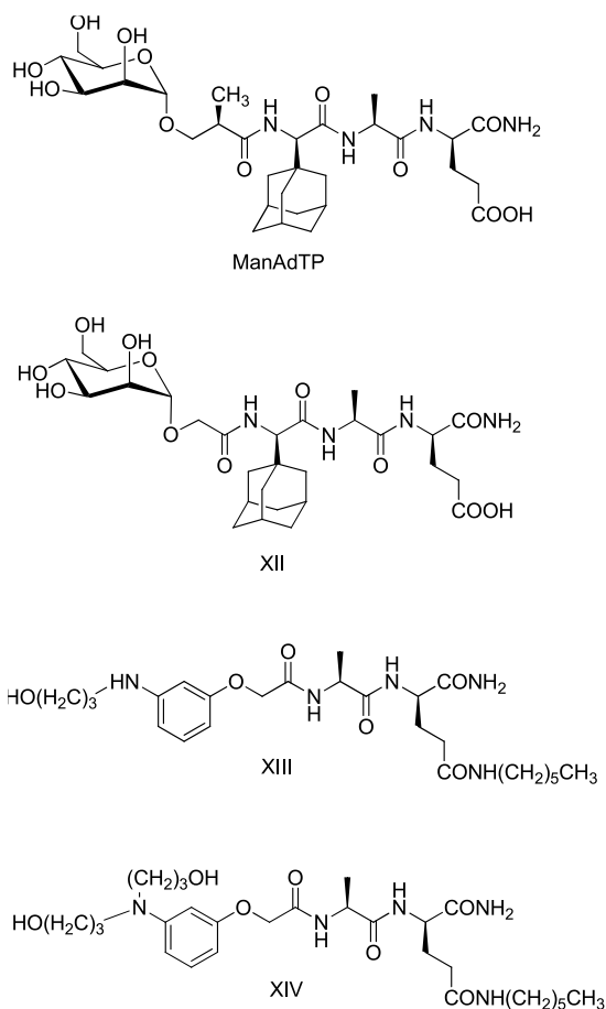
Figure 9. Perspective amphiphilic DMP derivatives.
