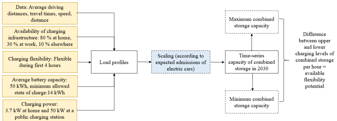
Figure 2. Approach for calculation of flexibility potentials due to flexible charging of electric vehicles according to Arnold et al. [60]
