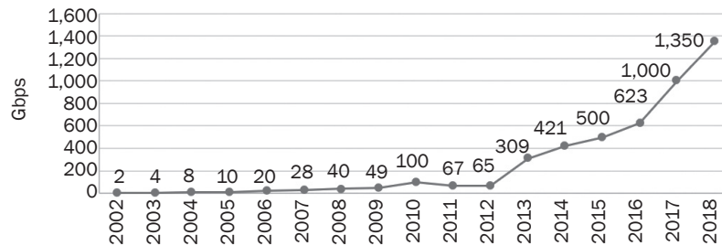
Figure 4 – Intensity of generated DDoS traffic over time period 2002-2018 [17, 27, 31]
