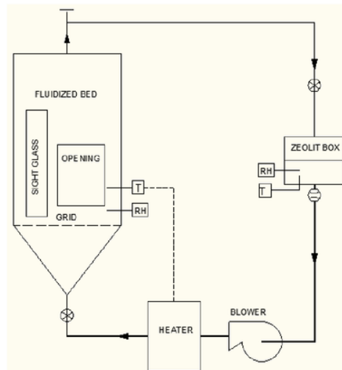
Gambar 1. Skema fluidized bed dryer sistem tertutup.
