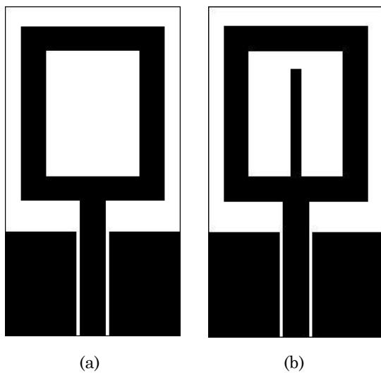
Fig. 2 – Design stages of the proposed antenna: (a) basic antenna structure (Antenna a), (b) proposed antenna (Antenna b)
